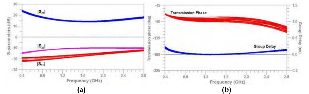
Fig. 17(a). S-parameters magnitudes and (b) transmission phase and group delay with a Monte Carlo analysis as a function of R , L , C and d .
