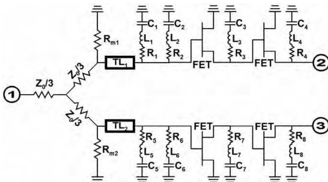
Fig. 19. Schematic of the simulated NGD active balun: Z_0 = 50 \, \Omega , R_1 = 83 \, \Omega , R_2 = 120 \, \Omega , R_3 = 22 \, \Omega , R_4 = 42 \, \Omega , R_5 = 40 \, \Omega , R_6 = 43 \, \Omega , R_7 = 12 \, \Omega , R_8 = 36 \, \Omega , R_{m1} = 120 \, \Omega , R_{m2} = 150 \, \Omega , L_1 = 1 \, \text{nH} , L_2 = 320 \, \text{pH} , L_3 = 270 \, \text{pH} , L_4 = 531 \, \text{pH} , L_5 = 3.3 \, \text{nH} , L_6 = 6.5 \, \text{nH} , L_7 = 1.3 \, \text{nH} , L_8 = 3 \, \text{nH} , C_1 = 2.8 \, \text{pF} , C_2 = 2.6 \, \text{pF} , C_3 = C_4 = 2.4 \, \text{pF} , C_5 = 0.6 \, \text{pF} , C_6 = 0.1 \, \text{pF} , C_7 = 0.7 \, \text{pF} , C_8 = 0.6 \, \text{pF} , TL_1 ( d_1 = 4.49 \, \text{mm} , Z_{c1} = 50 \, \Omega ), and TL_2 ( d_2 = 24.89 \, \text{mm} , Z_{c2} = 50 \, \Omega ) printed on a RF35 substrate ( \epsilon_r = 3.5 , h = 508 \, \mu\text{m} ), FETs: EC-2612 biased at V_{gs} = -0.1 \, \text{V} , V_{ds} = 3 \, \text{V} .
