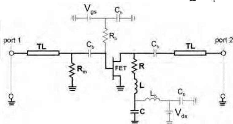
Fig. 10. Detailed schematic of the simulated NGD PS (biasing network in thin line): R_m = 51 \Omega , C_b = 22 \text{ nF} , L_b = 390 \text{ nH} , R_b = 1 \text{ k}\Omega , FET/EC-2612 ( V_{gs} = -0.1 \text{ V} , V_{ds} = 3 \text{ V} , I_{ds} = 30 \text{ mA} ) and TL ( w = 952 \mu\text{m} , d = 3.7 \text{ mm} ) printed on an FR4 substrate with relative permittivity, \epsilon_r = 4.3 , and thickness, h = 508 \mu\text{m} .
