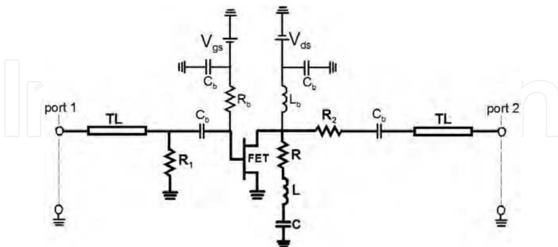
Fig. 14(a): Detailed schematic (biasing network in thin line) of the tested NGD PS : R_1 = 51 \, \Omega , R_2 = 22 \, \Omega , R = 33 \, \Omega , L = 4.7 \, \text{nH} , C = 1 \, \text{pF} , C_b = 22 \, \mu\text{F} , L_b = 220 \, \text{nH} , R_b = 1 \, \text{k}\Omega , FET (EC-2612 biased at V_{gs} = -0.1 \, \text{V} , V_{ds} = 3 \, \text{V} and I_{ds} = 30 \, \text{mA} ) and TL ( w = 952 \, \mu\text{m} , d = 6.2 \, \text{mm} ).
