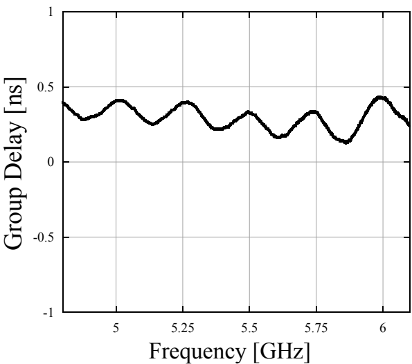
Fig. 18. Measured group delay in the frequency range 4.8 – 6.1 GHz.
