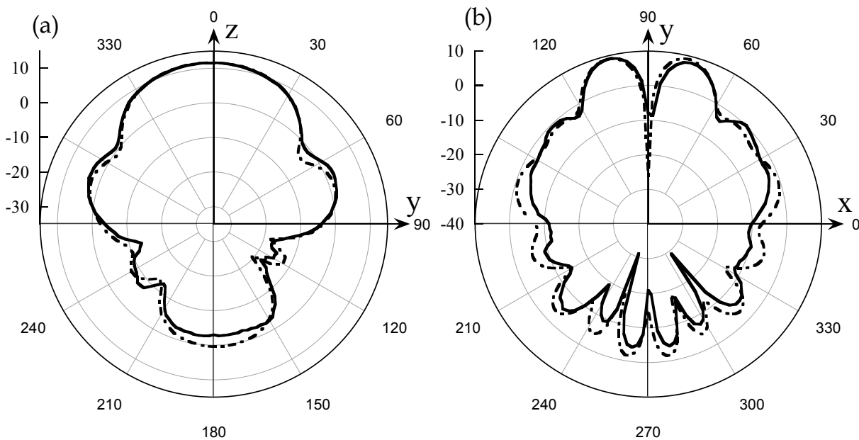
Fig. 24. Measured (solid line) and simulated (dashed-dotted line) radiation patterns for in-plane polarization at 7 GHz. (a) y - z plane, differential excitation. (b) x - y plane, port 1 and port 2 are excited with the same polarity, maximum gain is 9 dB. The results are reported in dB.
