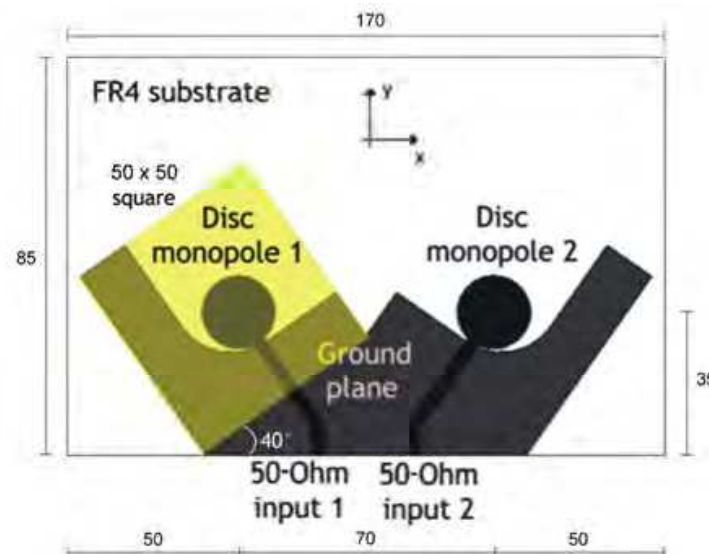
Fig. 19. Sketch of the differential UWB antenna: disc monopoles and microstrip lines (black), structured ground plane (dark gray) and the basic element of the array (yellow square) are depicted. The dimensions are in millimeters.
