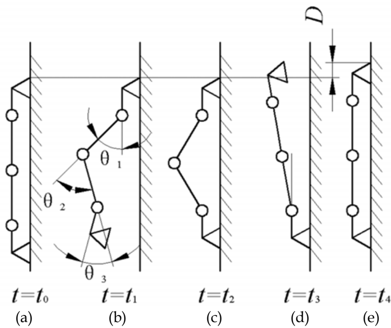
Fig. 7. The locomotion gaits of inchworm robot
