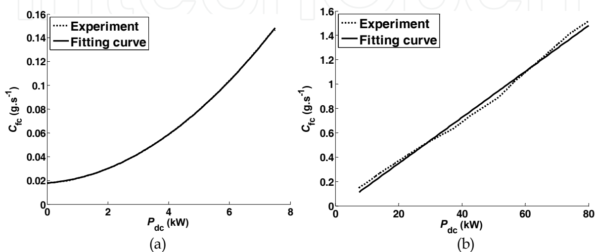
Fig. 4. (a) Relationship between fuel cell hydrogen consumption C_{fc} and DC/DC power P_{dc} when P_{dc} \leq 7.5 kW (b) Relationship between fuel cell hydrogen consumption C_{fc} and DC/DC power P_{dc} when P_{dc} > 7.5 kW
