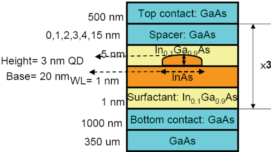
Fig. 5. The schematic 3 period of QD heterostructure with cross-sectional lens-shaped geometry.
