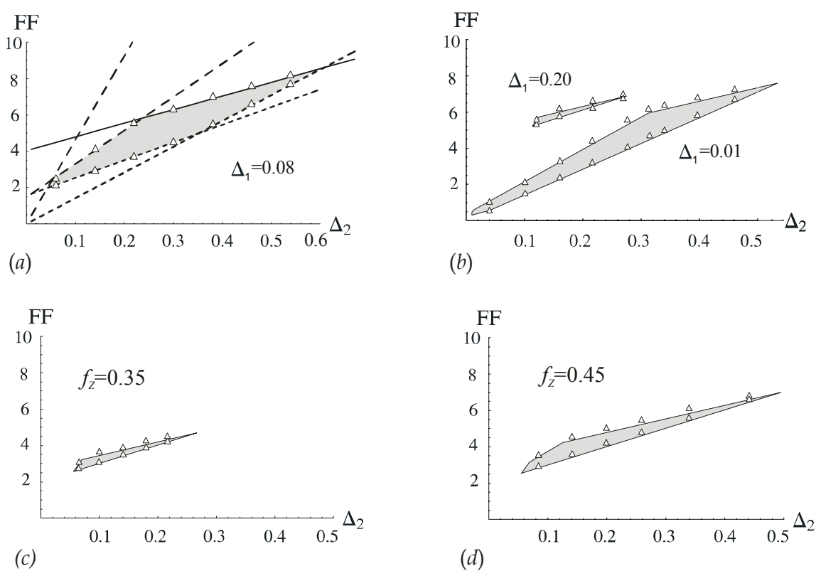
Fig. 7. (a) Set of constraints from which the correct operation region is derived. Grey area depicts feasible values of FF vs. \Delta_2=f_B - f_Y for \Delta_1=f_A - f_B = f_Y - f_Z=0.08 and f_Z=0.6 . Triangles delimit the region given by HSPICE simulations with nonlinear RTD models. Feasible (\Delta_2,FF) pairs for (b) \Delta_1=0.01 and \Delta_1=0.20 , f_Z=0.6 . (c) \Delta_1=0.1 , f_Z=0.35 . (d) \Delta_1=0.1 , f_Z=0.45 .
