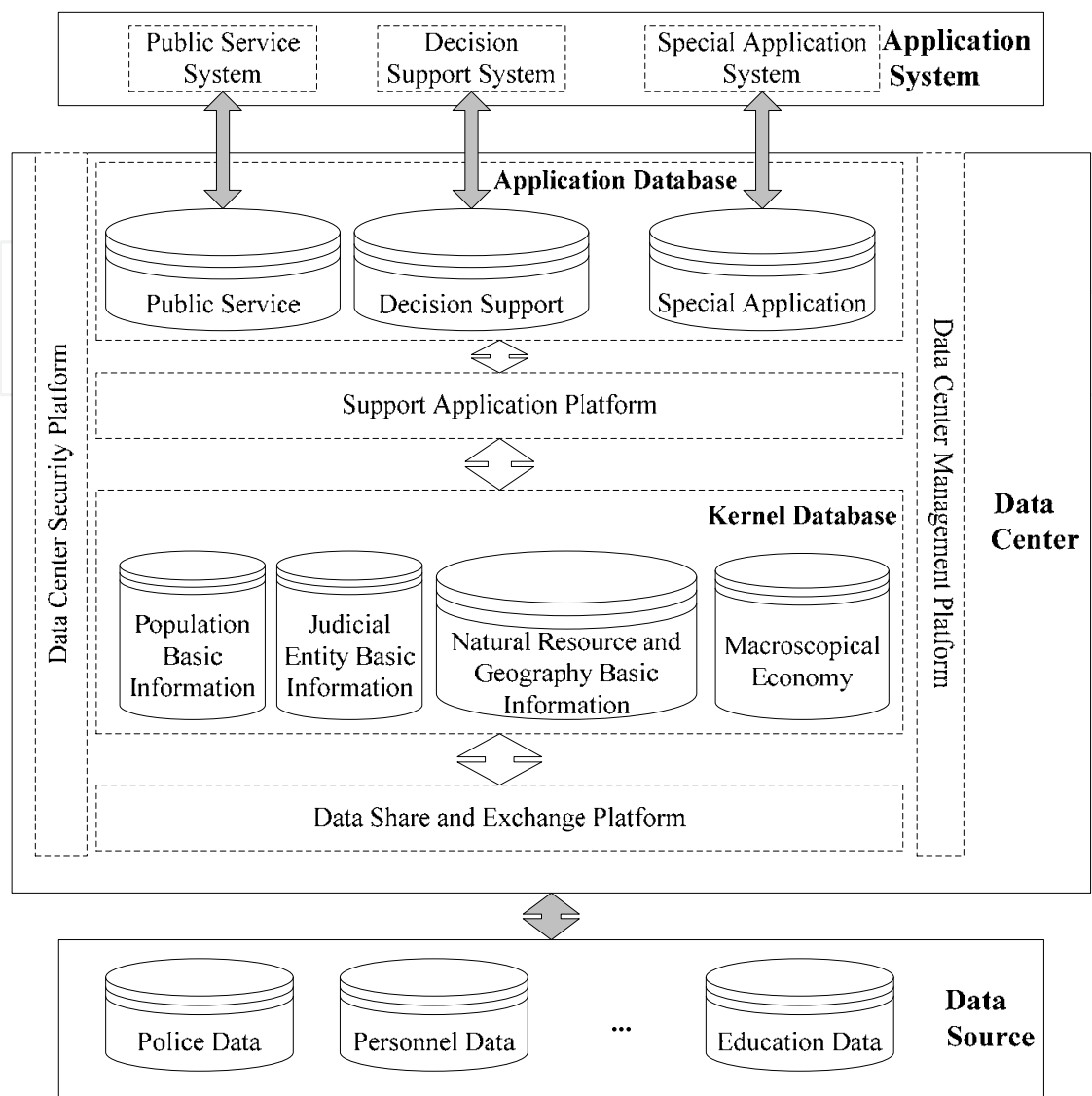
Fig. 8. Architecture of Data Centre
