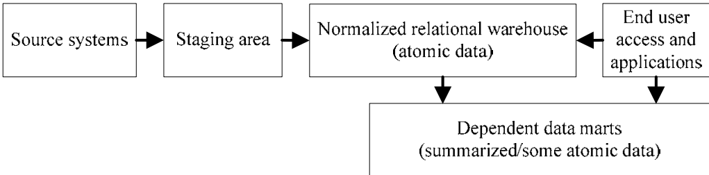
Fig. 3. The hub and spoke architecture
