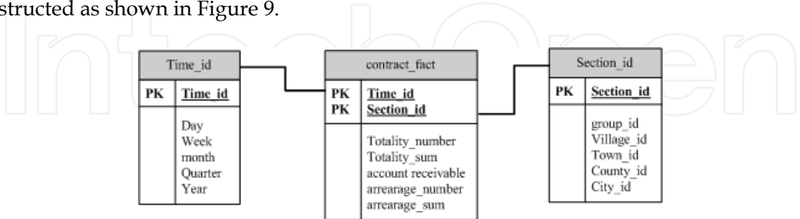
Fig. 9. Star Schema of Contract Data
