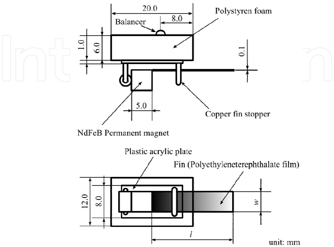
Fig. 16. Shape and dimension of the micro swimming mechanism
