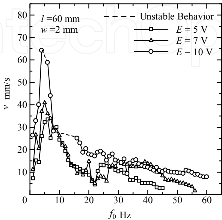
Fig. 18. Frequency characteristics of the micro swimming mechanism
