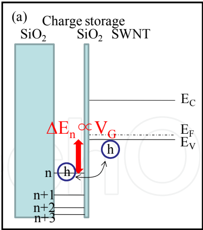
Fig. 12. (a) Schematic model of charge storage. When the charge storage energy level is coincident with the top of the valence band owing to applied gate voltage, the carrier goes and comes between them through the barrier with tunneling. The exiting probabilities of the carrier at the charge storage and the valence band depend on the relative height of their energy levels under equilibrium condition.
