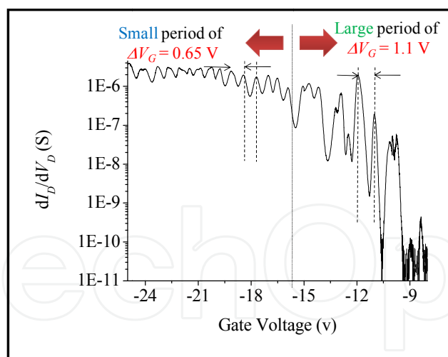
Fig. 2. (a) Differential conductance dI_D/dV_D characteristic as a function of V_G at 7.3 K. Two frequencies of oscillation were observed, which were \Delta V_G = 1.1 V and 0.65 V.
