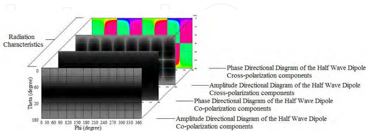
Fig. 9. Radiation characteristics of the half-wave dipole in 2-D.
