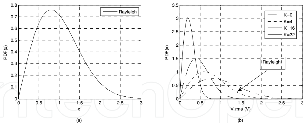
Fig. 17. a) Rayleigh density function and b) Rayleigh PDF for the several K values
