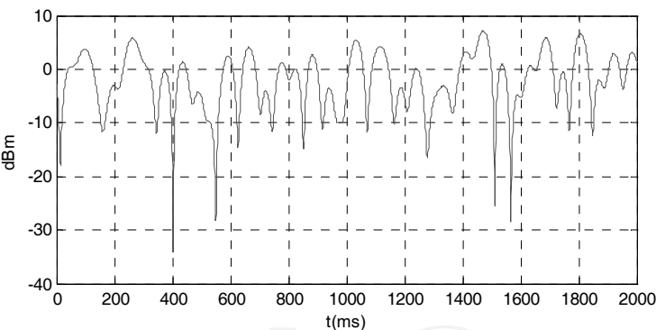
Fig. 7. Signal at the antenna terminals under multipath
