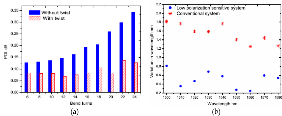
Fig. 26. (a) PDL of the fiber filters with 90° twist and its comparison with the PDL of the filters without twist (b) Comparison of wavelength errors in a low polarization system vs. conventional system
