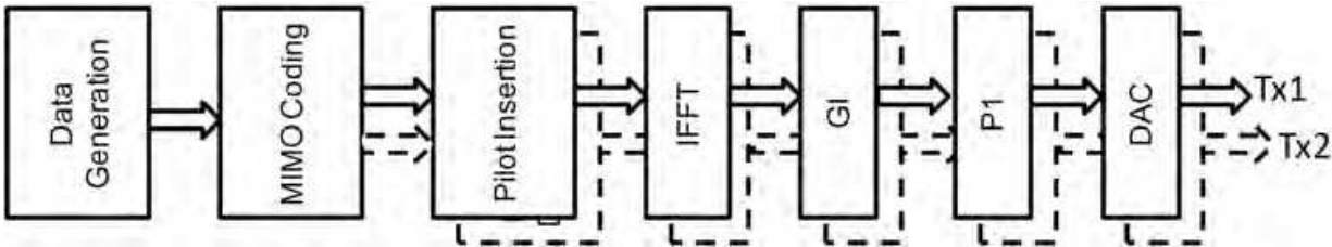
Fig. 12. Block diagram of the transmitter signal processing
