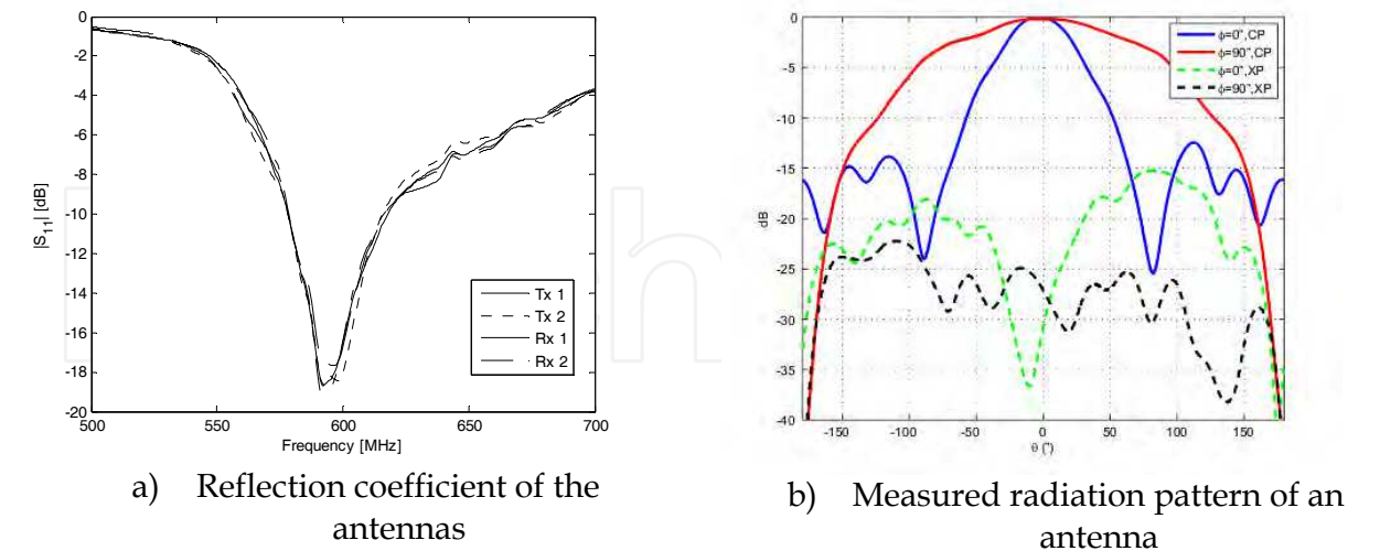
Fig. 18. Antenna performances
