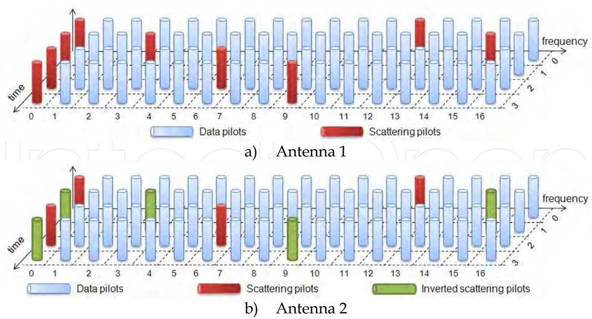
Fig. 16. Scattered pilots distribution
