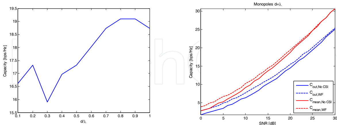
a) Capacity of monopoles array as a function of spacing with a SNR=20dB b) Comparison of monopoles capacity with a spacing of \lambda , as a function of SNR and CSI
