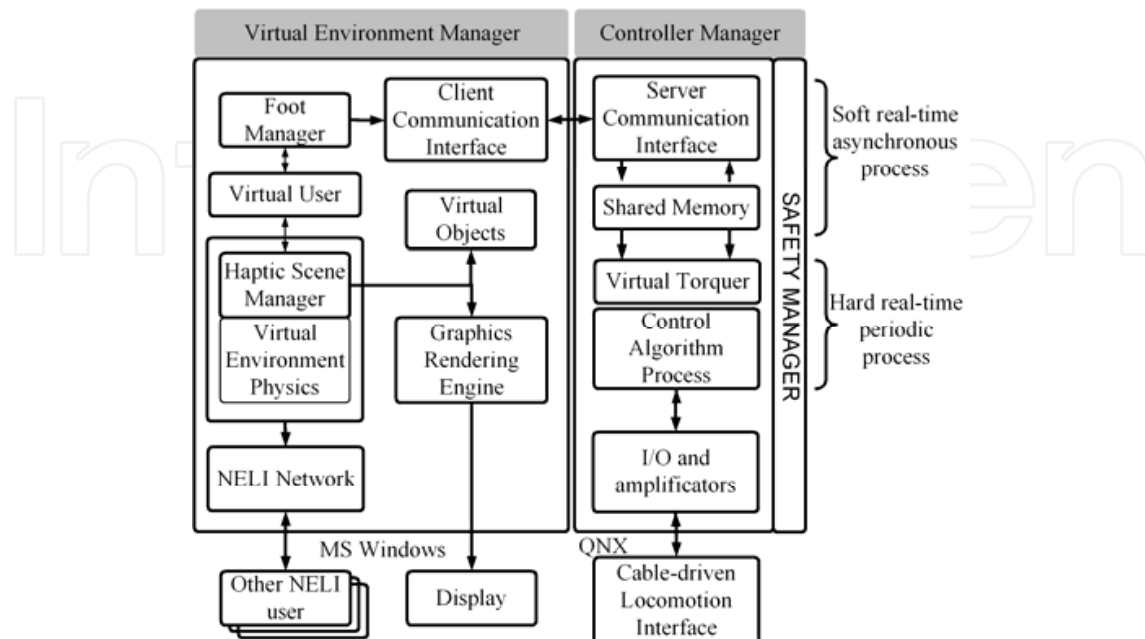
Fig. 3. Software architecture
