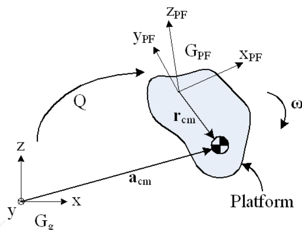
Fig. 5. Reference frame of the platform
