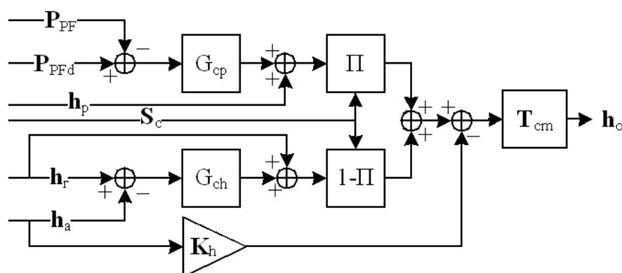
Fig. 6. Admittance/Impedance/Null Force Hybrid Control
