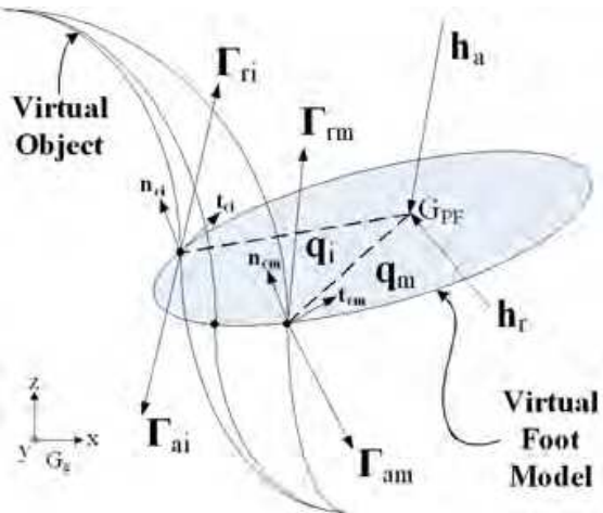
Fig. 8. Collision model with action and reaction wrenches
