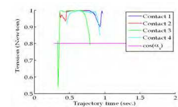
Fig. 14. Friction cone condition
