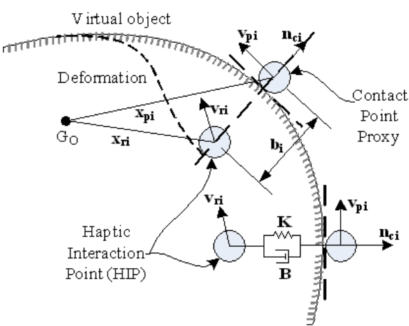
Fig. 9. Contact point proxy for each contact points with the respective penetration
