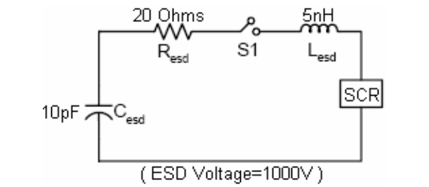
Fig. 15. Equivalent circuit of CDM Model
