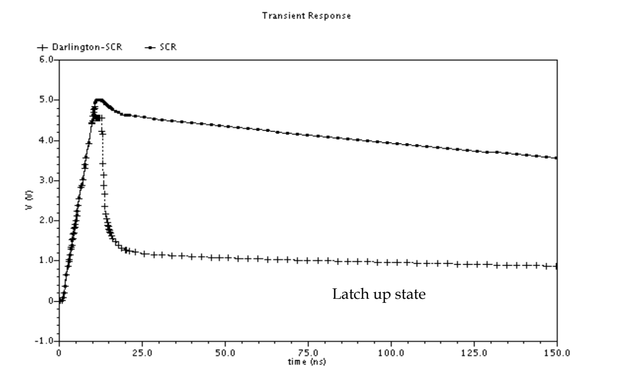
Fig. 35. Trigger characteristic comparison of normal SCR and Darlington SCR when the base current is 0.37mA
