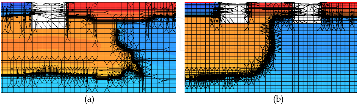
Fig. 5. (a) Bad boundary shape, (b) Good boundary shape
