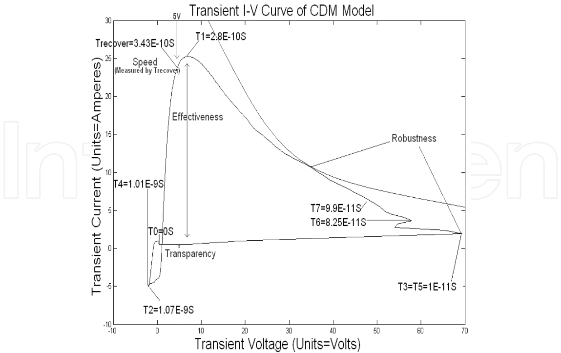
Fig. 23. Ransient I(t) versus transient V(t) of SCR-based ESD protection device
