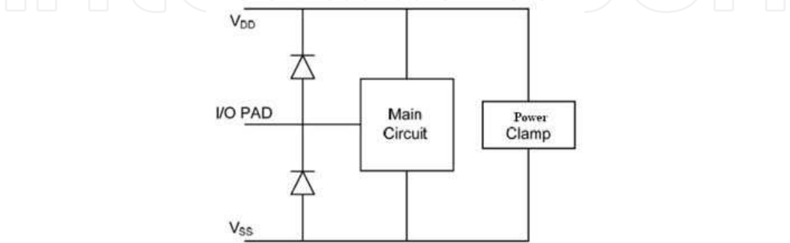
Fig. 24. Rail-based ESD protection scheme with power clamp
