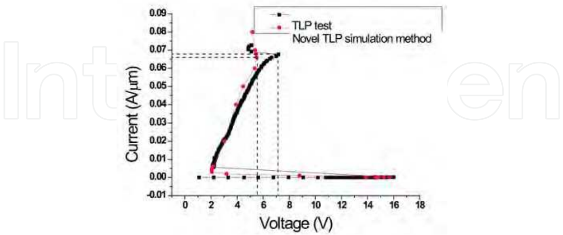
Fig. 13. I_{t2} obtained from novel TLP simulation and that from TLP test
