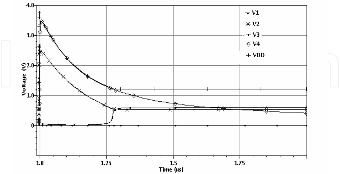
Fig. 28. Simulated voltage at the different node under 5KV HBM ESD event
