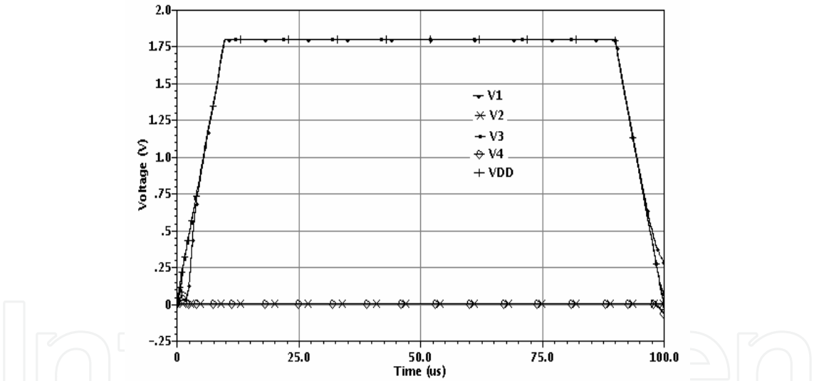
Fig. 29. Simulated voltage at the different node at fast power on state
