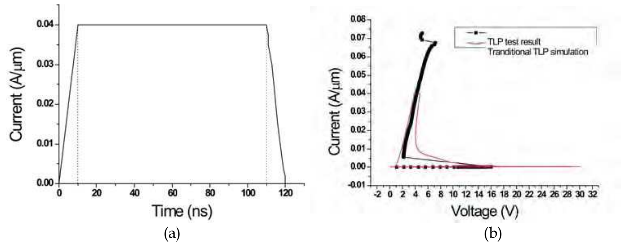
Fig. 9. (a) Current pulse imposed on the simulated structure (b) I-V characteristic obtained from TLP test and traditional TLP simulation method
