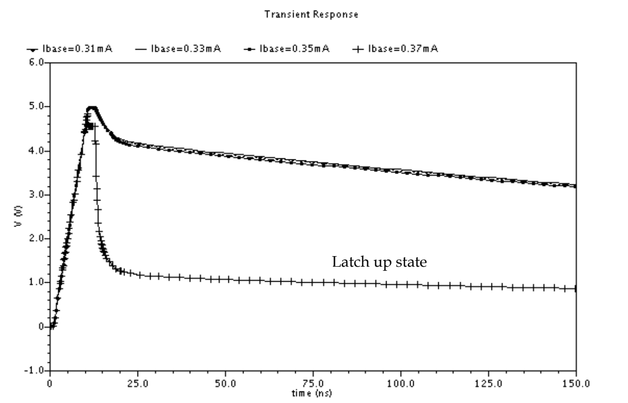
Fig. 34. Simulation results of Darlington SCR triggering characteristic
