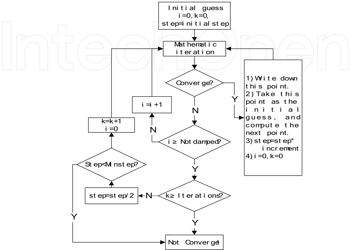
Fig. 2. Device simulation flow
