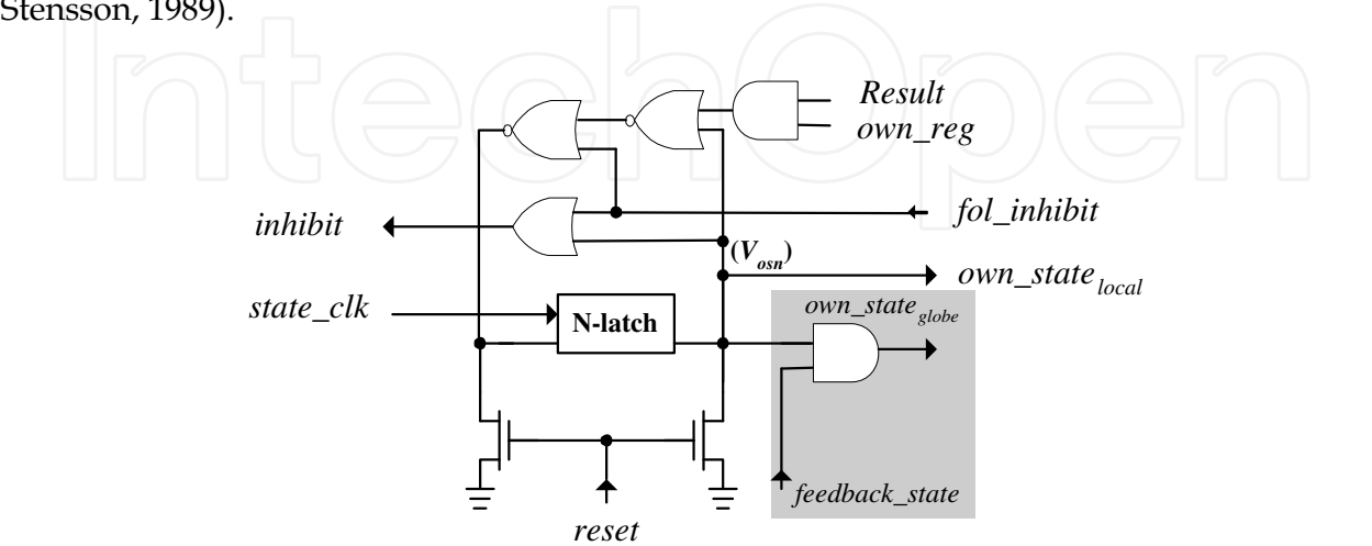
Fig. 11. Status block.
