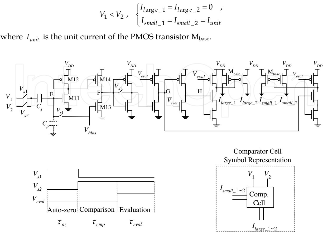
Fig. 19. 1.2-V auto-zero comparator, clock, and symbol representation.
