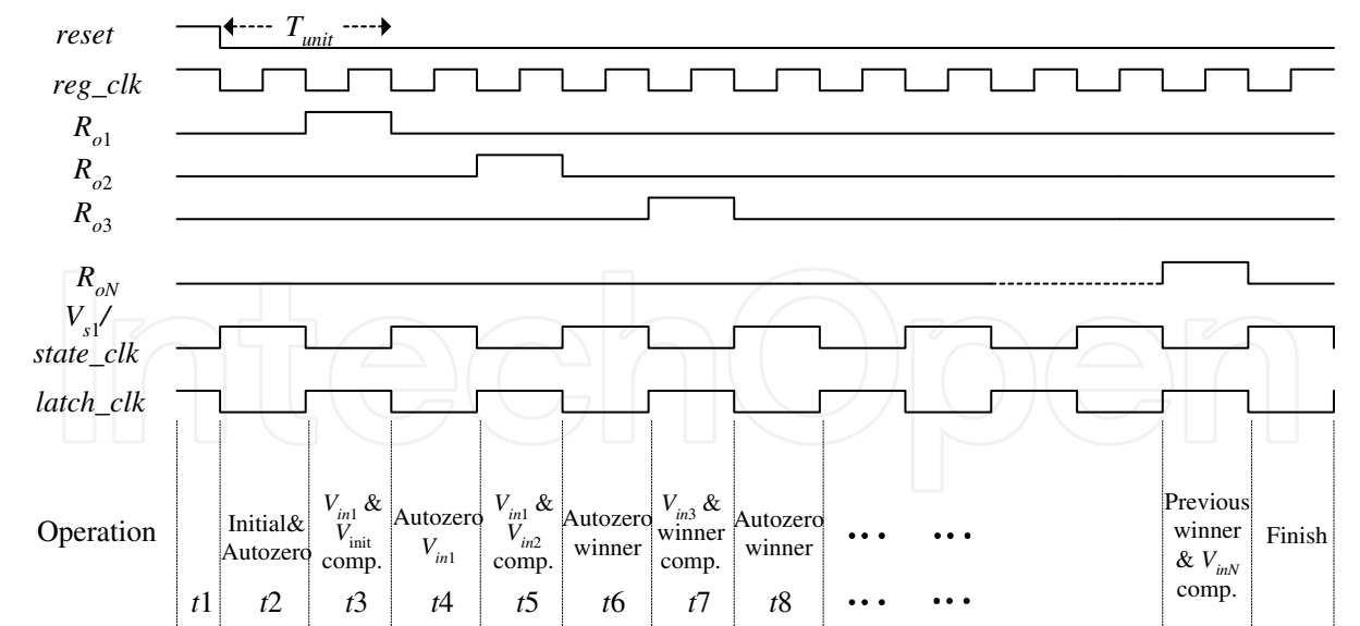
Fig. 10. Clock waveforms. Then, at t2 , the V_{s1} clock turns high (auto-zero phase) to sample the initial voltage (0 V or V_{DD} ) at node cap\_comn . Next, at t3 , R_{o1} turns high to sample voltage V_{in1} . At this time, the clock V_{s1} turns low (comparison phase) to compare the V_{in1} with the initial sampling voltage, and the compared result is stored in the N-latch of the first status block. The state of the N-latch is logic 1 if the variable is the winner. At t4 , the present winner V_{in1} is sampled again. At t5 , a new comparison between previous winner V_{in1} and V_{in2} is performed. At t6 , the winner (the result for the V_{in1} and V_{in2} comparison) is sampled again. After this procedure, a new comparison between the present winner and V_{in3} is performed. The procedure continues until comparison of all the input voltages is completed. Ultimately, only one state V_{osn} ( n=1, \dots, N ) in these cells is logic 1 for WTA/LTA indication; others are logic 0. Therefore, a WTA or a LTA operation has been accomplished. Figure 11 shows the status block. Figure 12 shows the control_switch block. It receives an input variable and controls the transmission gate to sample input level. A true single-phase latch composed of an N-latch and a P-latch is used to reduce the clock skew issue (Yuan & Stensson, 1989).
