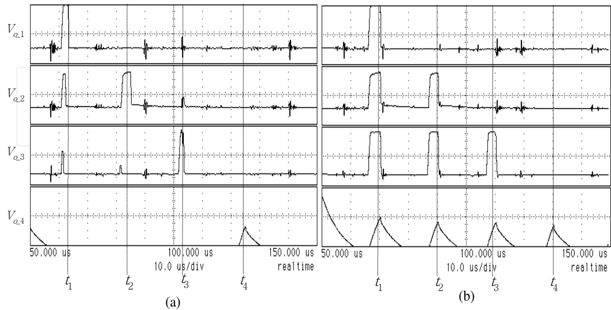
Fig. 22. The measurement results of (a) rank-order (b) k -WTA operations.
