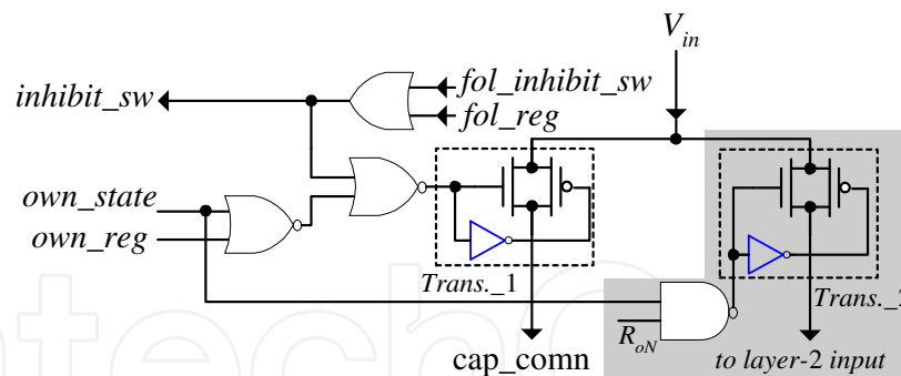
Fig. 12. Control_switch block.
