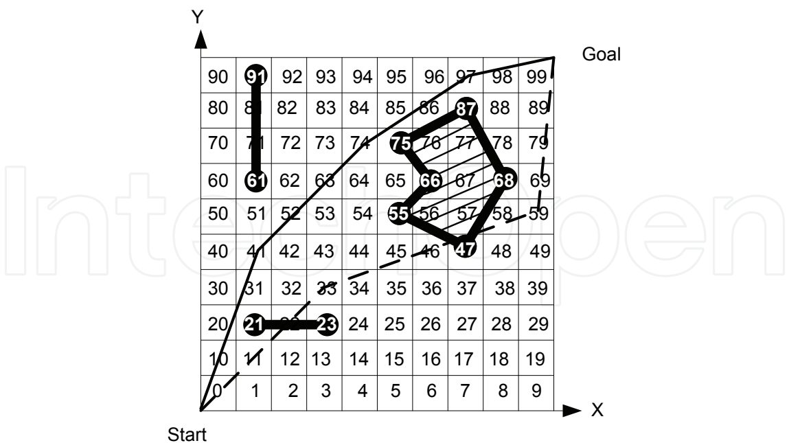
Fig. 5. Environment presented in form of occupancy grid. Numbers denote different nodes. Bold lines: obstacles; solid lines: feasible path; dashed line: unfeasible path.
