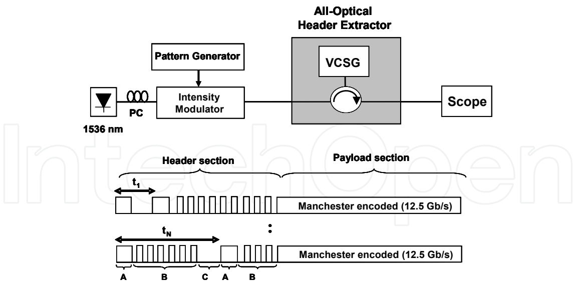
Fig. 11. The set-up and format of the packets used in the AO-HE experiment.
