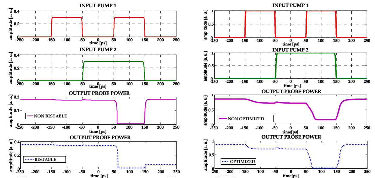
Fig. 19. Left: dynamic NAND operation with NRZ pulses at 10 Gb/s for pump and probe signals tuned at two different resonances ( \alpha_{ns}d= 0.005 , \alpha_0d = 0.25 , P_{pb}=P_{sat} ); the output probe power for non bistable (solid line) and bistable (dashed lines) cases, are shown. Right: dynamic NAND operation relative to the static characteristics of Fig 18; output probe power for non optimized (solid line) and optimized (dashed lines) cases, are shown
