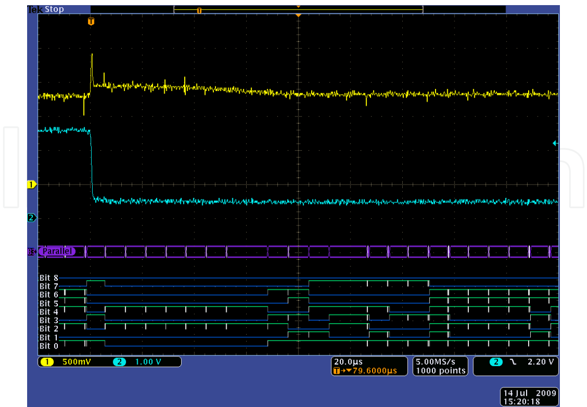
(a) H: 20µs/div.
