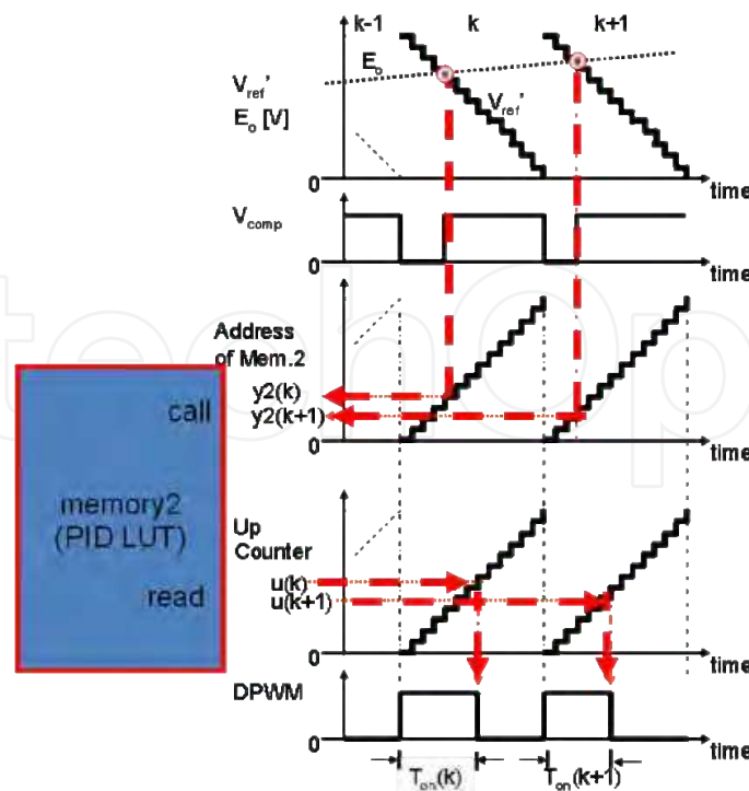
Fig. 5. Theoretical waveforms.
