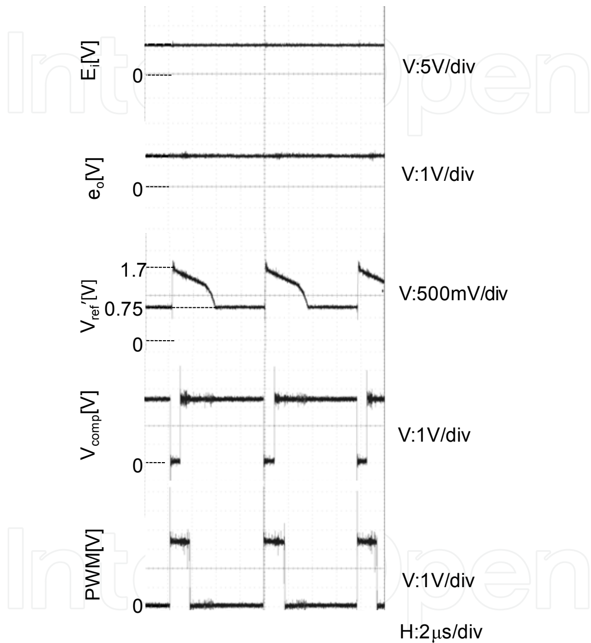
Fig. 8. Experimental waveforms
