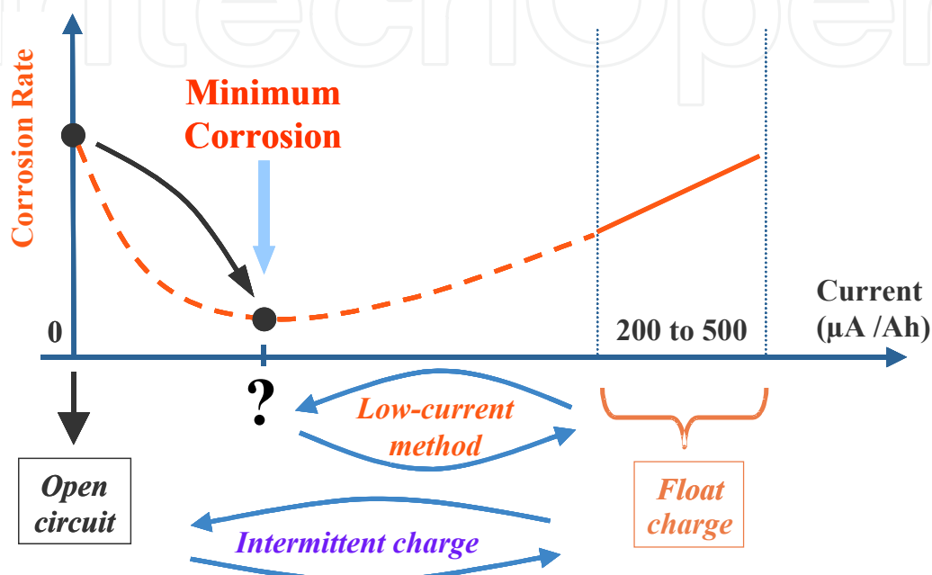
Fig. 7. Low-current method is derived from intermittent charge: open circuit periods are replaced by low currents, whose values are smaller than float current (200 to 500 \mu\text{A/Ah} ). Battery should be in the minimum corrosion zone
