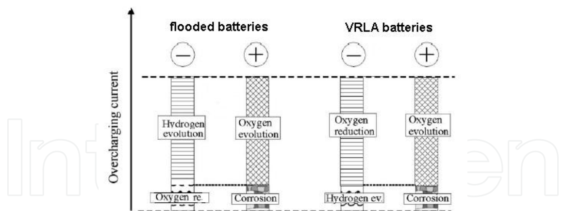
Fig. 2. Description of equal float current flows through both electrodes in the normal conditions at flooded batteries and VRLA batteries (supposing that the recombination efficiency at the VRLA battery is 100%)
