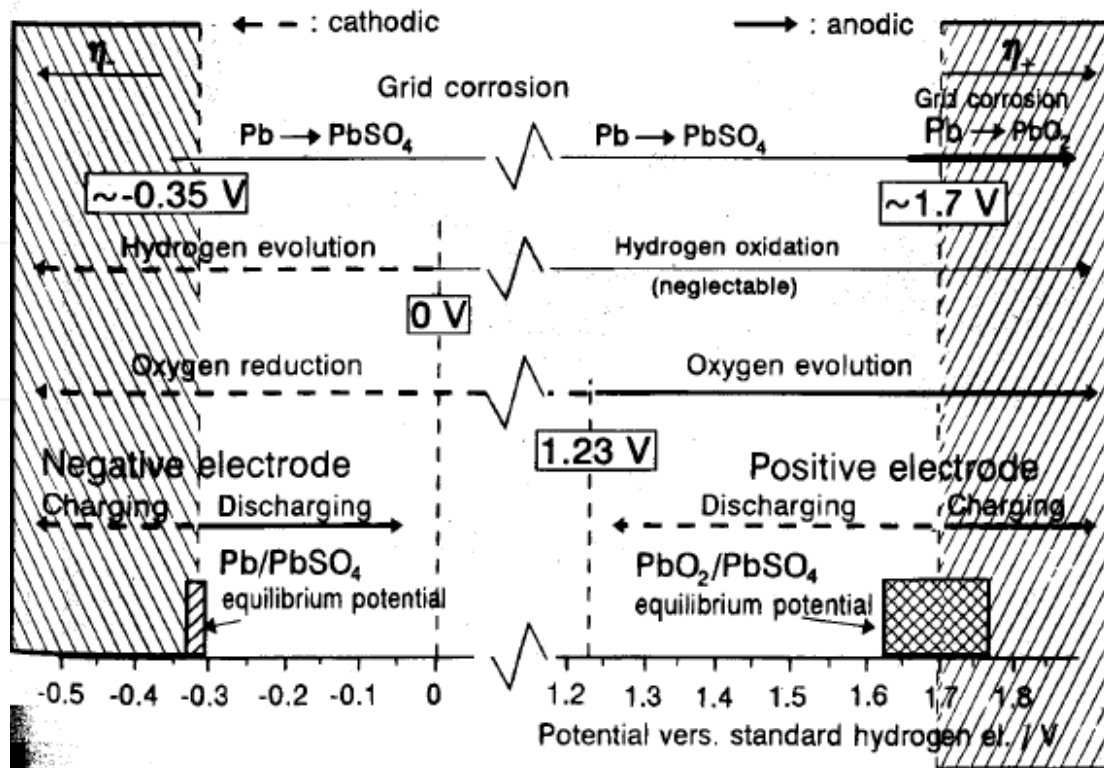
Fig. 1. Reactions that occur in lead acid batteries dependent on electrode potential. Equilibrium potentials of charge-discharge reactions ( \text{Pb/PbSO}_4 and \text{PbSO}_4/\text{PbO}_2 ) are presented in columns, because they depend on the acid concentration. (Berndt and Teutsch, 1996)
