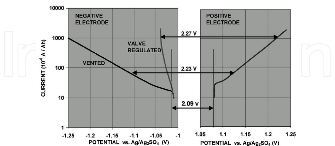
Fig. 3. Polarization curves of positive and negative electrodes, when measured against silver-silver sulfate reference electrodes. This figure demonstrates that the positive electrodes of valve-regulated batteries are subjected to much higher potentials than the positive electrodes in vented batteries (Ruetschi, 2003)
