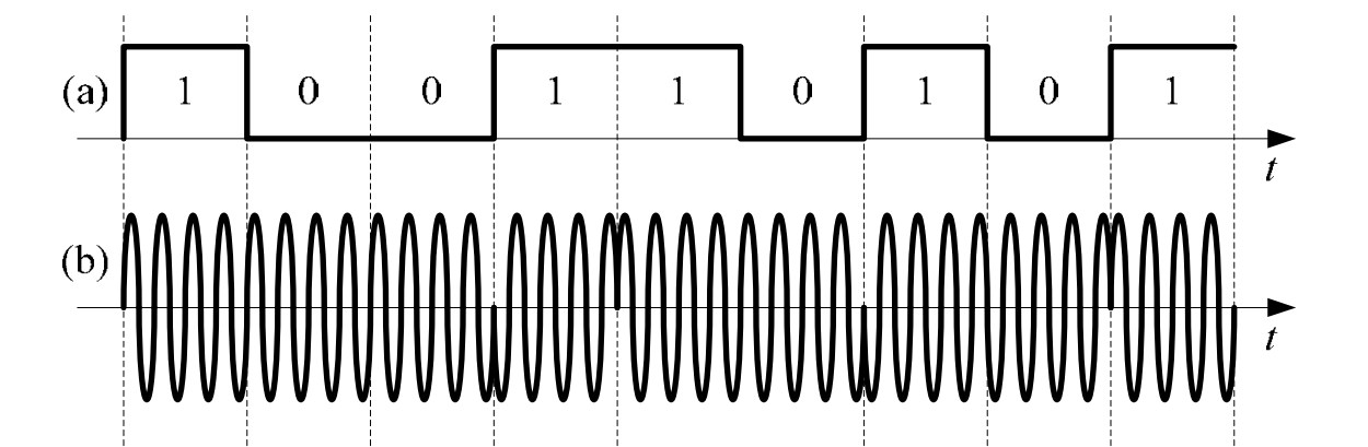
Fig. 4. Example of DPSK modulation format, (a) binary signal, and (b) DPSK modulated signal
