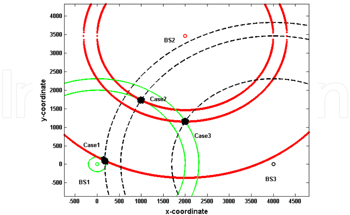
Fig. 9. Layout of the mobile localization geometry used to test the accuracy of the AML algorithm.
