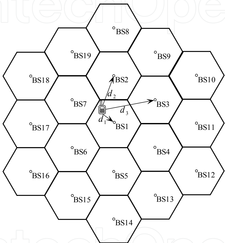
Fig. 3. Cellular network model, with center cell and two tiers of interfering cells.
