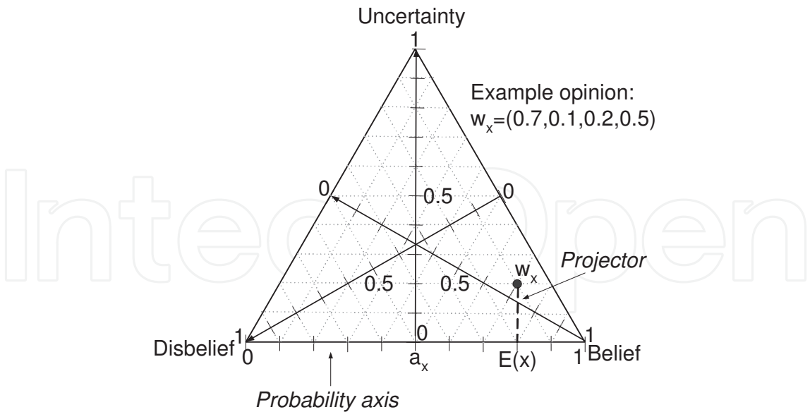
Fig. 1. Opinion triangle with an example opinion (Jøsang, 2001).
