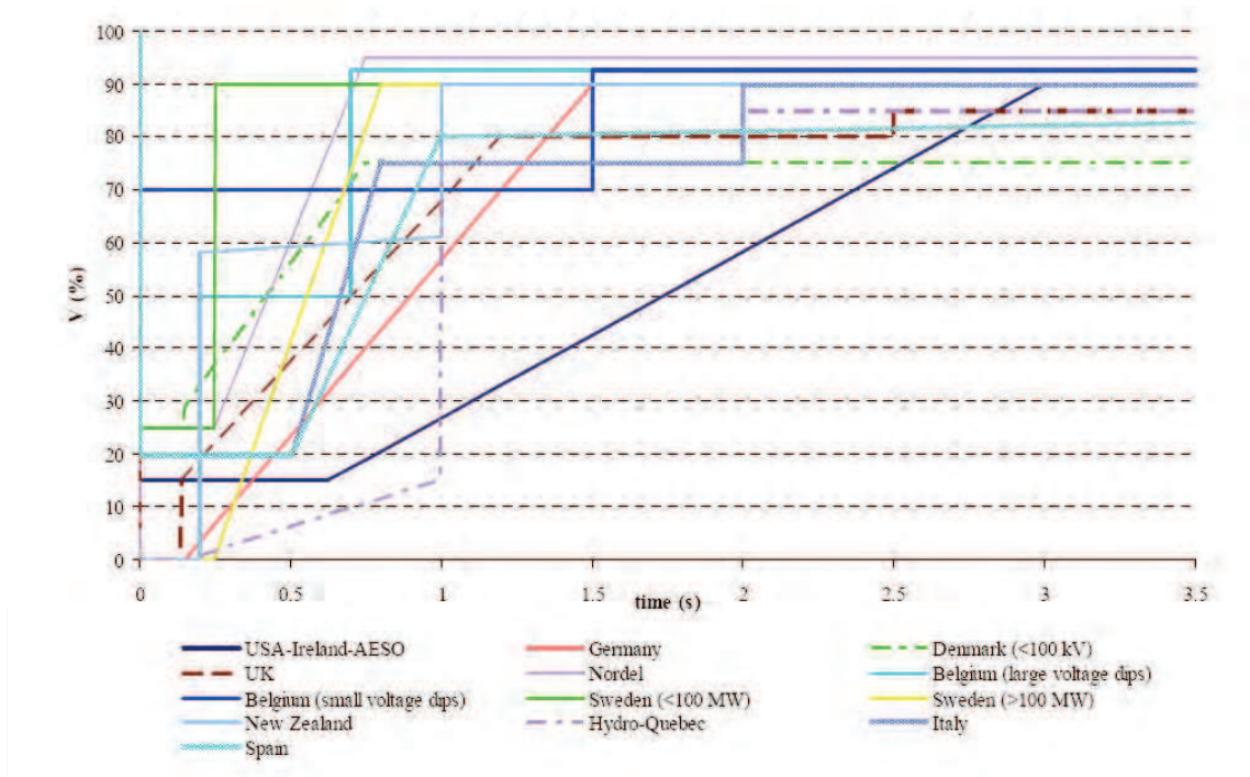
Fig. 2. LVRTF requirements for various grid codes (Tsili et al, 2009)
