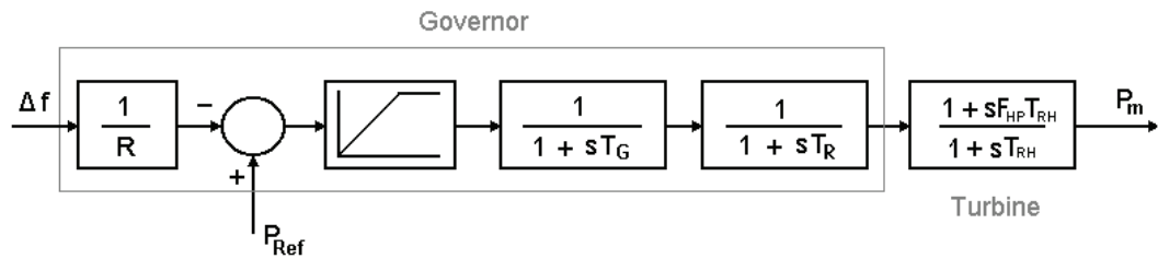
Fig. 9. Steam speed control system \Delta f , is the per unit frequency change ( f_o=50\text{Hz} ) P_m , is the mechanical power of the steam turbine.
