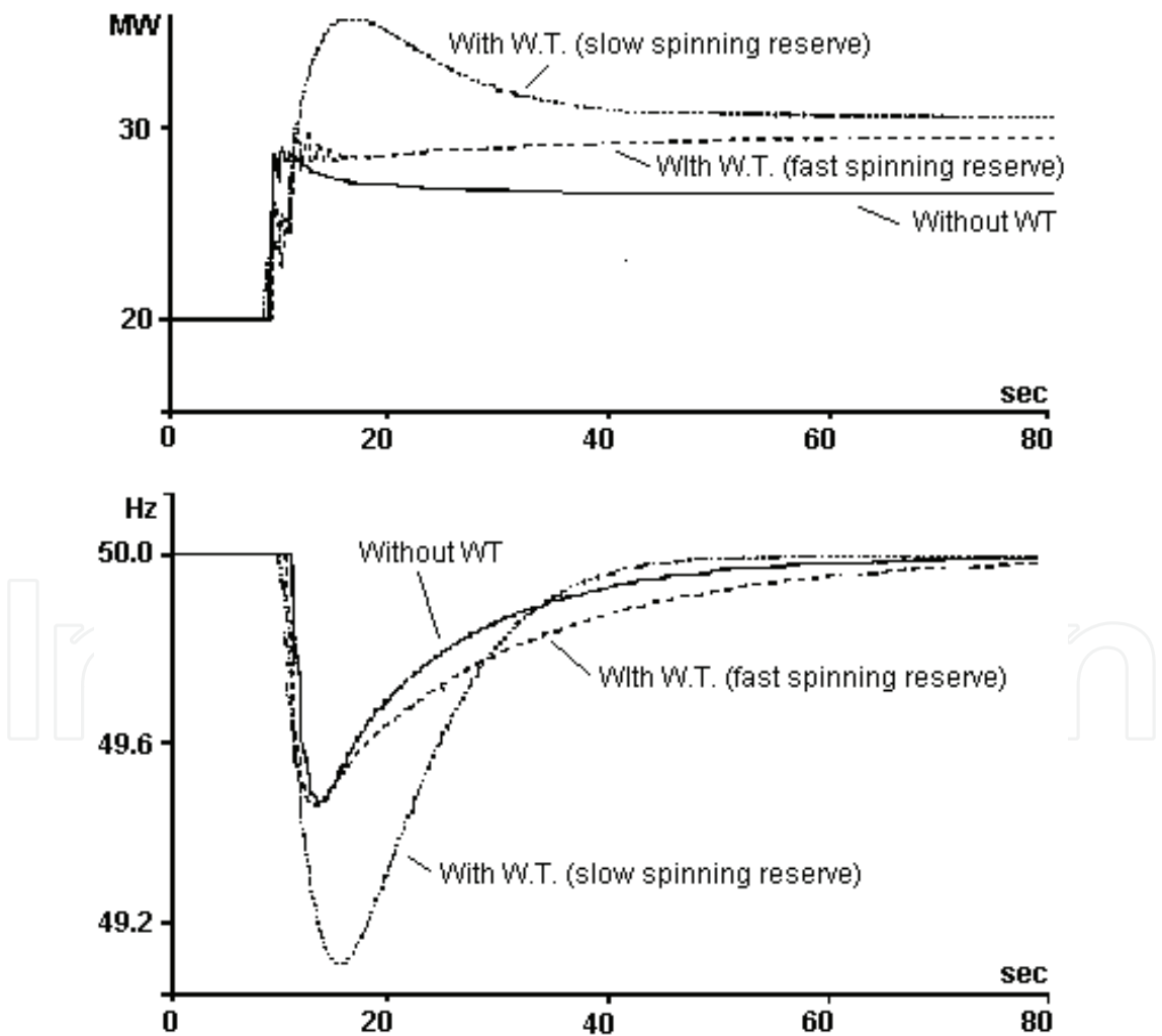
Fig. 15. Frequency and power change
