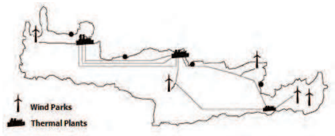
Fig. 5. Power plants and wind parks locations
