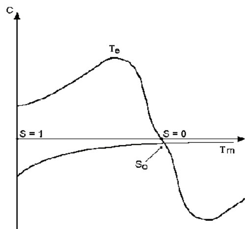
Fig. 11. Intersection of electrical and mechanical torque
