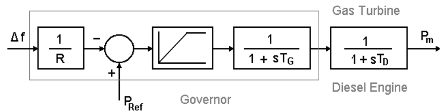
Fig. 8. Diesel-Gas speed control system \Delta f , is the per unit frequency change ( f_o=50\text{Hz} ). P_m , is the mechanical power of the diesel motor. R , is the droop of the speed governor.
