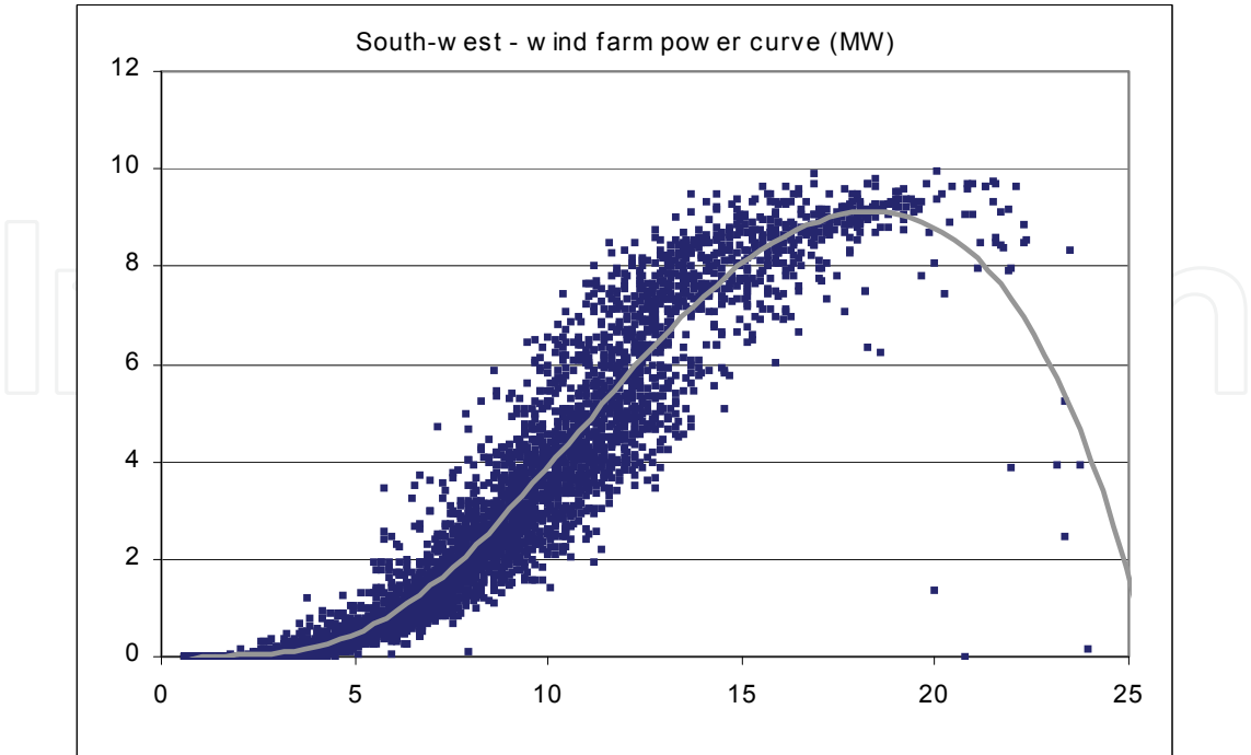
Fig. 12. Wind farm power curve and measures
