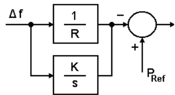
Fig. 10. Addition of integrating control block
