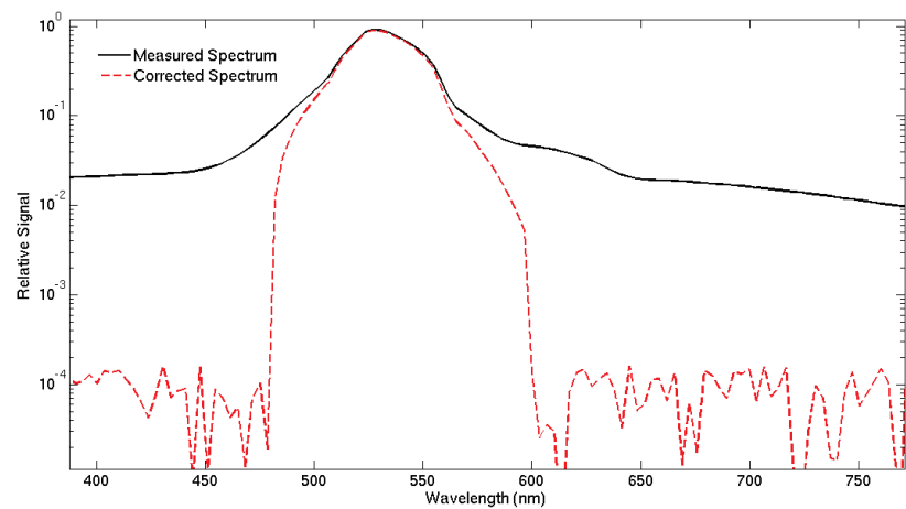
Fig. 4. Spectral stray-light correction applied to the miniature hyperspectral CMOS-array spectrometer in Figure 3, using a broadband source with a bandpass filter. Normalized measured and corrected signals. The y-axis is a logarithmic scale.
