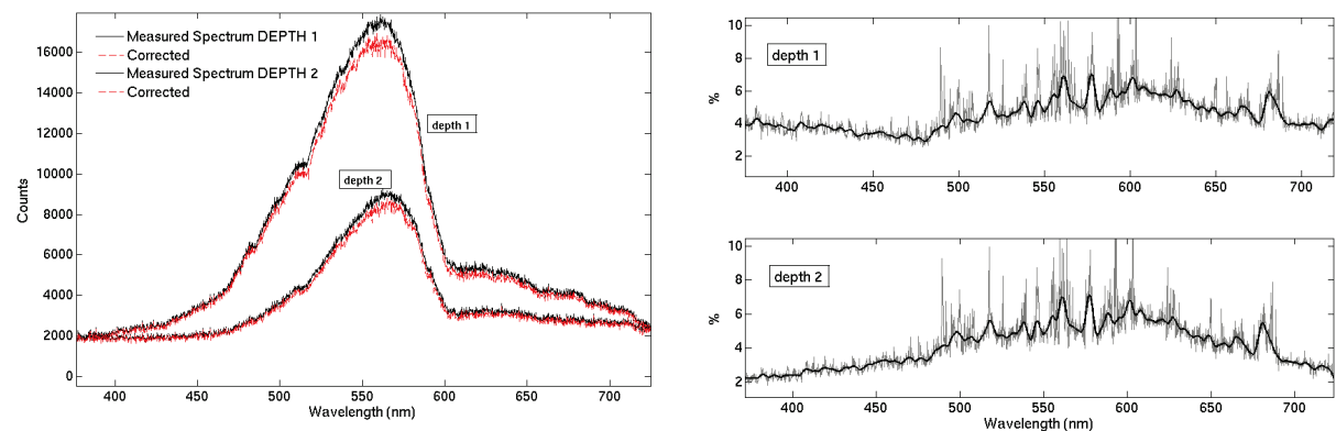
Fig. 5. (Left) Spectral stray-light correction applied to field underwater light measurements at two depths, acquired by a miniature hyperspectral CCD-array spectrometer. (Right) Difference in percentage between measured and corrected signals at each depth.
