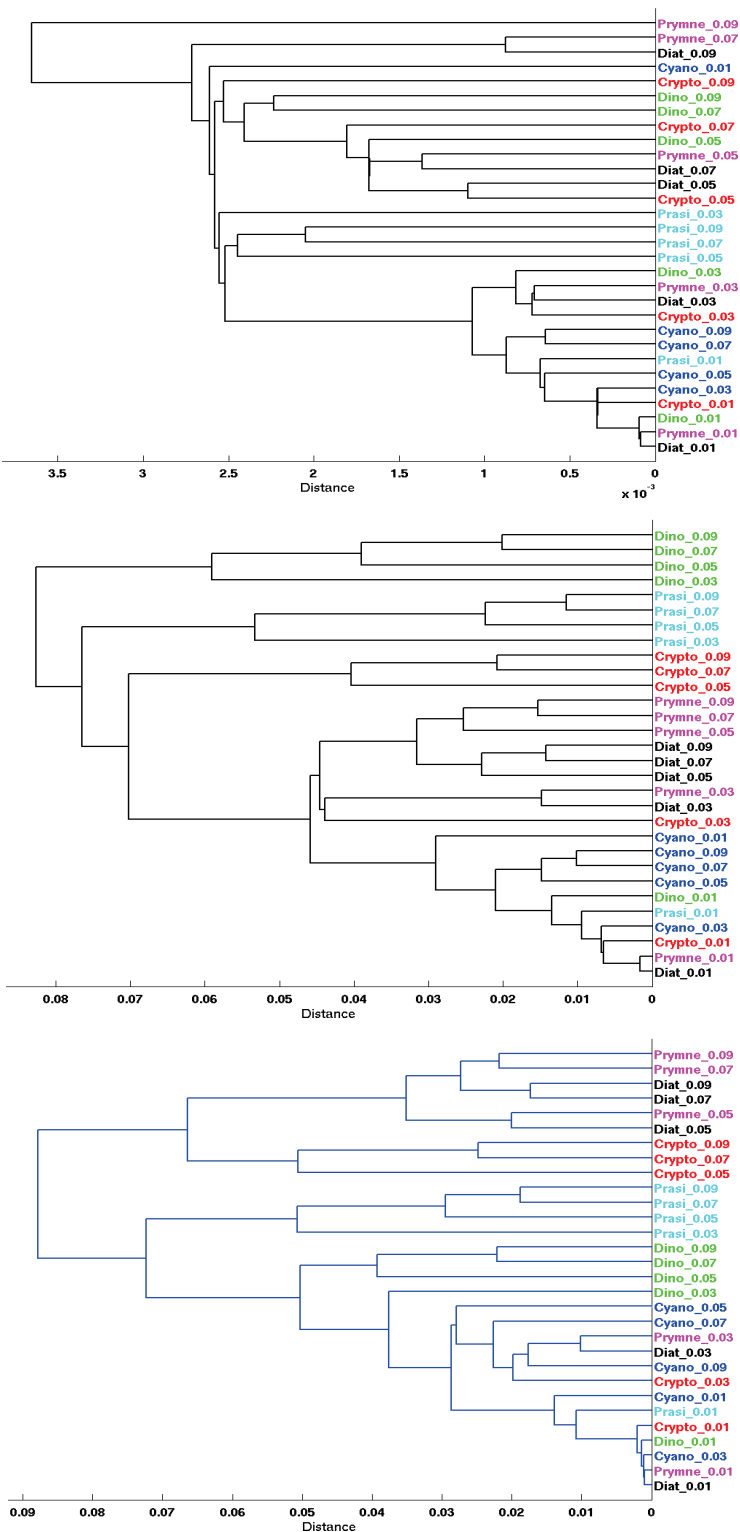
Fig. 10. Cluster analyses based on: (top) raw hyperspectral normalized R_{rs}(\lambda) , (centre) second derivative of hyperspectral normalized R_{rs}(\lambda) spectra and (bottom) second derivative of hyperspectral normalized R_{rs}(\lambda) spectra using analyzing parameters that are too coarse (i.e. derivative band separation and smoothing filter size).
