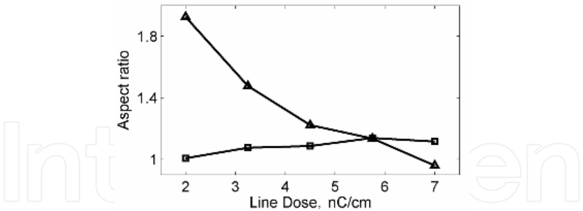
Fig. 9. Aspect ratios for the interline gaps (triangles) and PMMA lines (squares) as a function of the exposure dose, determined from cross-sectional SEM images for 70 nm pitch gratings fabricated using 30 keV electrons. Other process conditions were as in Fig. 8.
