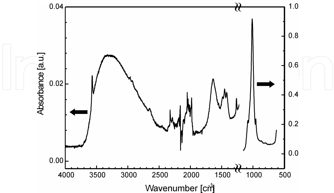
Fig. 9. FTIR spectrum of pure HAp nanorods.
