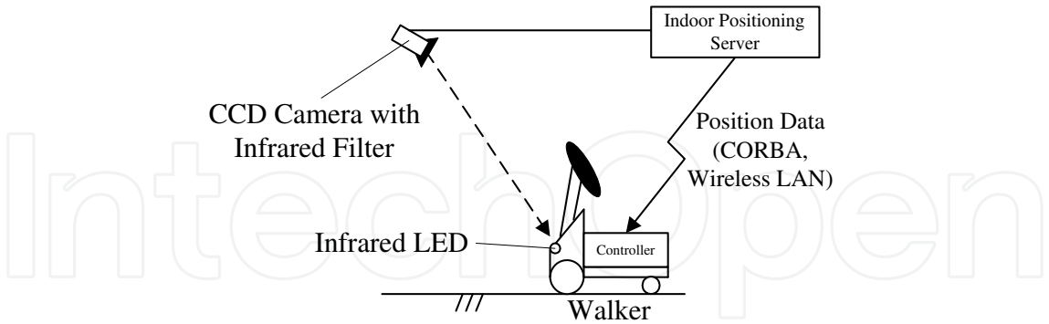
Fig. 11. The indoor positioning system.
