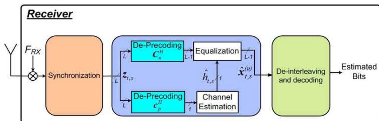
Fig. 4. Channel estimation scheme based on spread pilot
