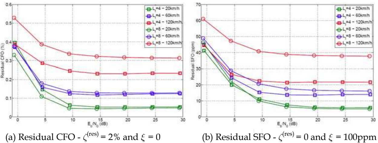
Fig. 12. Residual CFO and SFO after the 2nd synchronization stage - 16QAM data symbols - TU6 channel - L_f = 4
