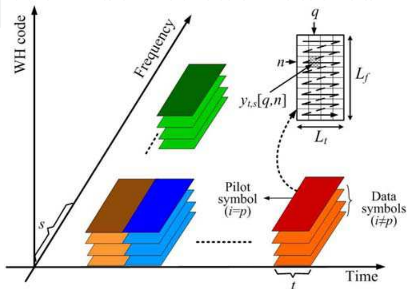
Fig. 3. 2D Spreading Scheme
