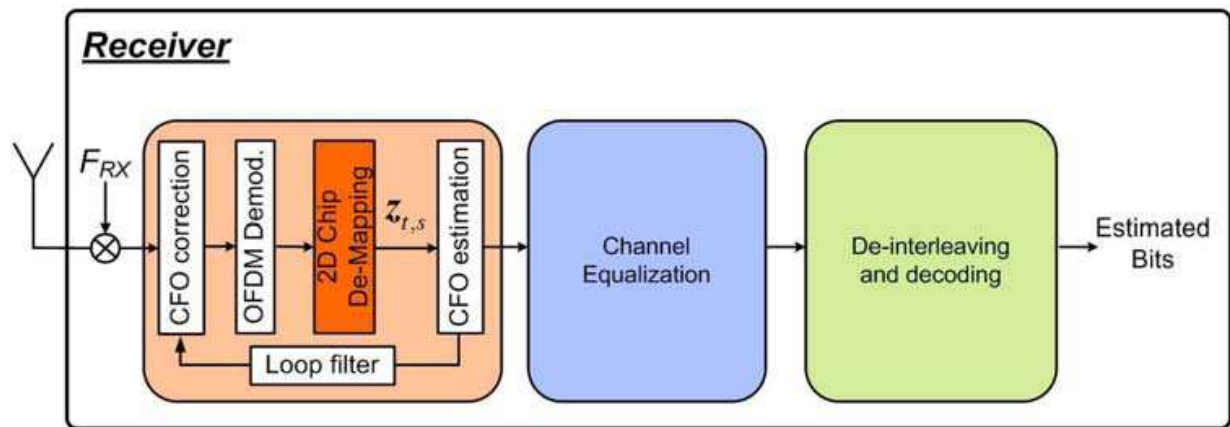
Fig. 9. Fine CFO estimation scheme before despreading function
