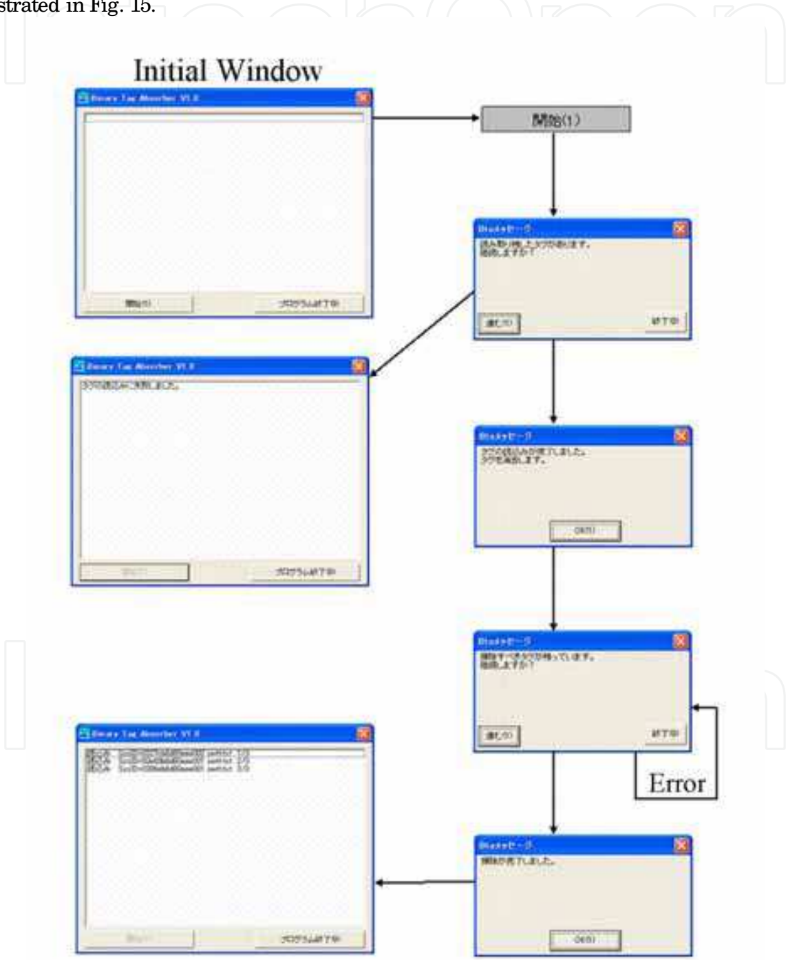
Fig. 15. Screen State Transition Diagram of the Binary Data Retrieval and Merge Functions
