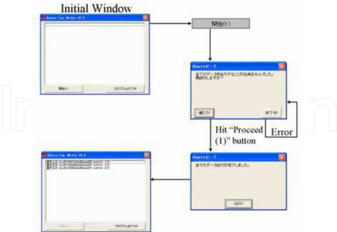
Fig. 14. Screen State Transition Diagram of the Binary Data Division Write Functions
