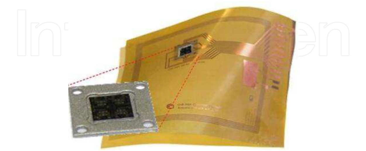
Fig. 10. First prototype of COF gas sensor integration.
