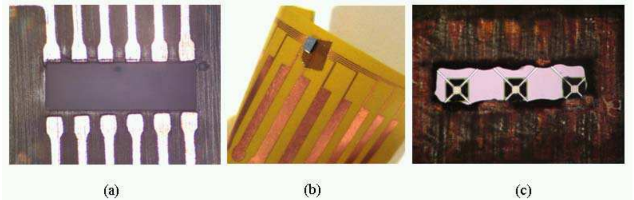
Fig. 5. (a) Flexible substrate fabricated to prove the viability of ACA flip chip assembly of ULPHP. (b)ULPHP chip assembled on the flexible substrate (c) View of the sensor membranes exposed to the air throw the ablated window.
