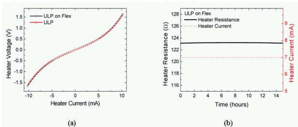
Fig. 6. (a) Comparison of resistance measurements between ULPHP (red) and encapsulated ULPHP (black). Each curve is the average of 6 different heaters within the test die. (b) Electrical short-term stability of the ACA flip chip bonding. The heater resistance does not change significantly during 15 hours of hotplate operation at 7 mA.
