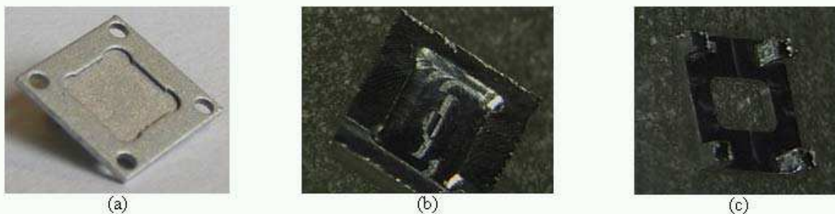
Fig. 8. (a) Stiffener 10 x 10 mm 2 ; (b) Stiffener 2.5 x 2.5 mm 2 ; (c) Cap 2.5 x 2.5 mm 2 .
