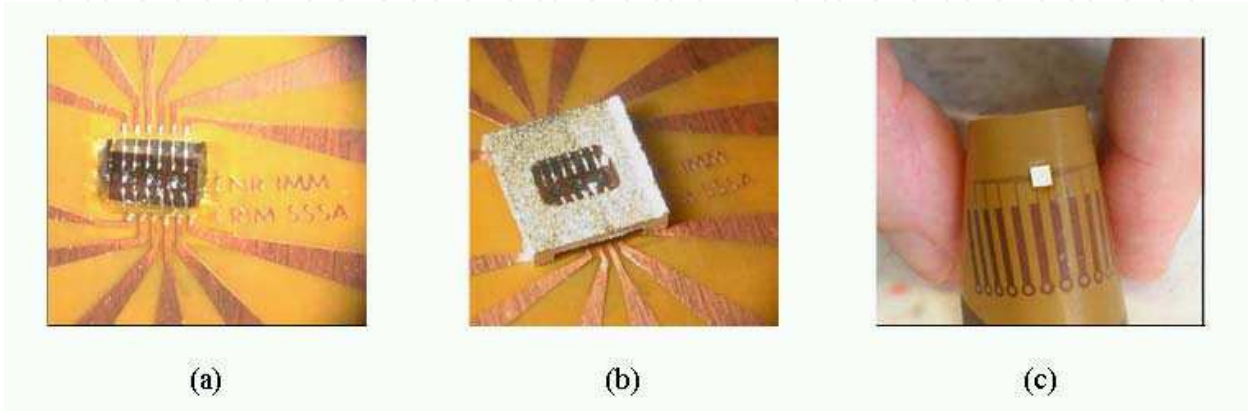
Fig. 11. Final prototype of ULP gas sensor array die integrated on flex. (a) wire-bonded array on stiffener. (b) array covered by protection cap. (c) effect of the stiffener during bending of the flex tag.
