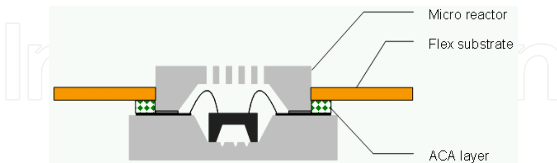
Fig. 12. Proposed all silicon MST solution using a silicon micro reactor chamber embedded into the flexible substrate. The bonding can be done by ACA flip chip bonding.
