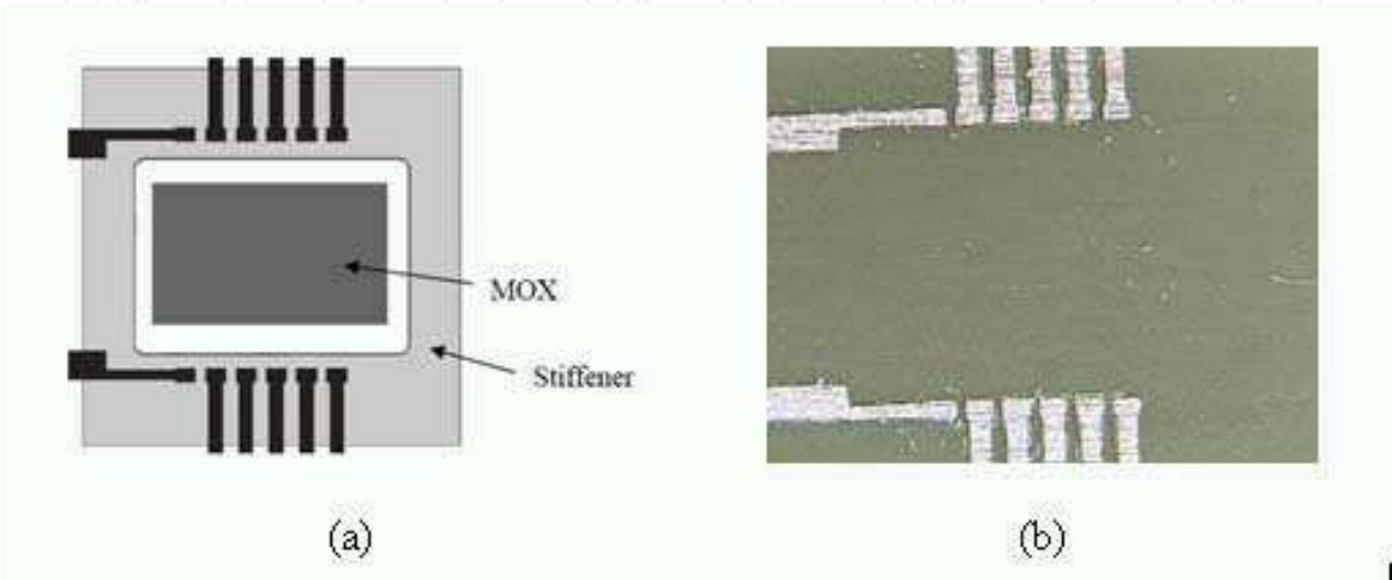
Fig. 9. (a) Assembling scheme; (b) Flexible substrate fabricated to prove the viability of COF wire bonding.
