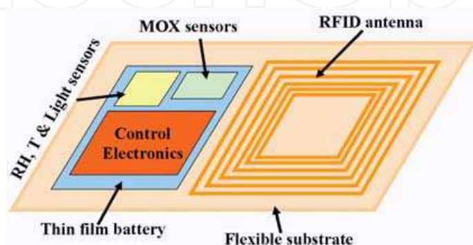
Fig. 1. Main functional blocks of the FTM inlay for food logistics.
