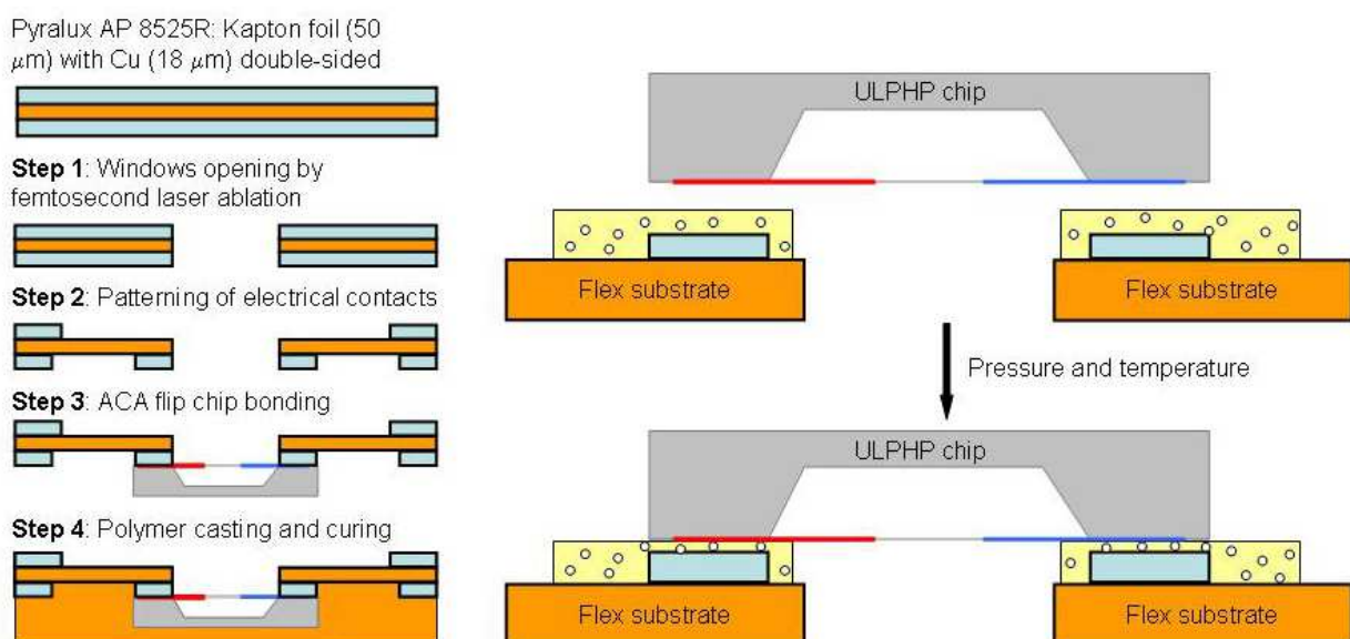
Fig. 4. (a) Process design for the MOX sensor integration. (b) Schematic view of the thermo-compression bonding using ACAs. Conductive particles are trapped between the flexible circuit and the chip pads.
