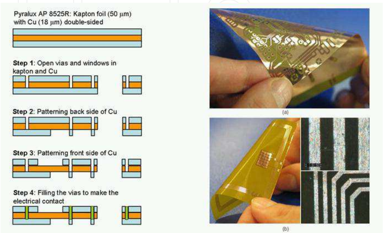
Fig. 2. Process design for flexible substrates fabrication, left image. Photographs and microscope images of the flexible circuit (a) and the flexible antenna (b). Detail of the copper tracks of the inductor.
