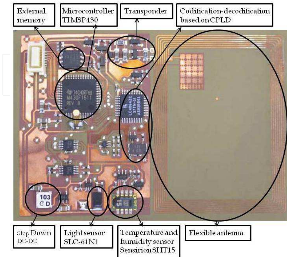
Fig. 3. FTM prototype including relative humidity, temperature and light sensors and a flexible antenna. A credit card size was chosen for the tag.
