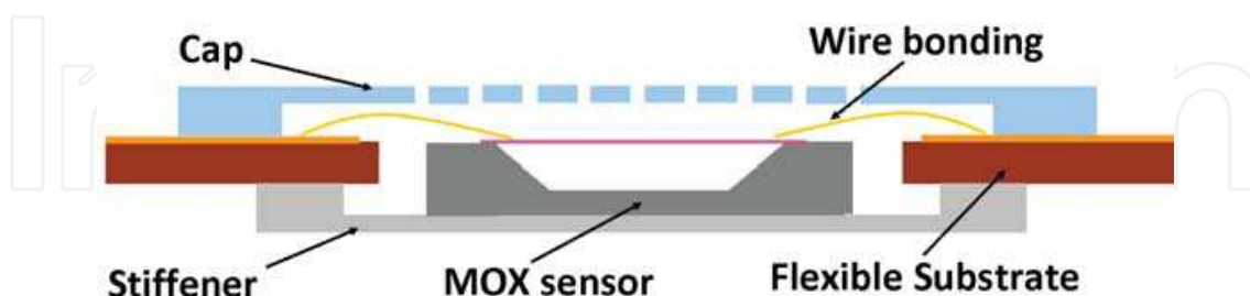
Fig. 7. Schematization of the chip-on-Flex structure.
