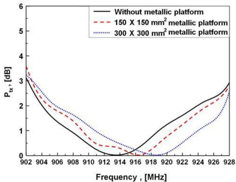
Fig. 4.5 Measured power bandwidth versus for different sizes of the metallic platforms
