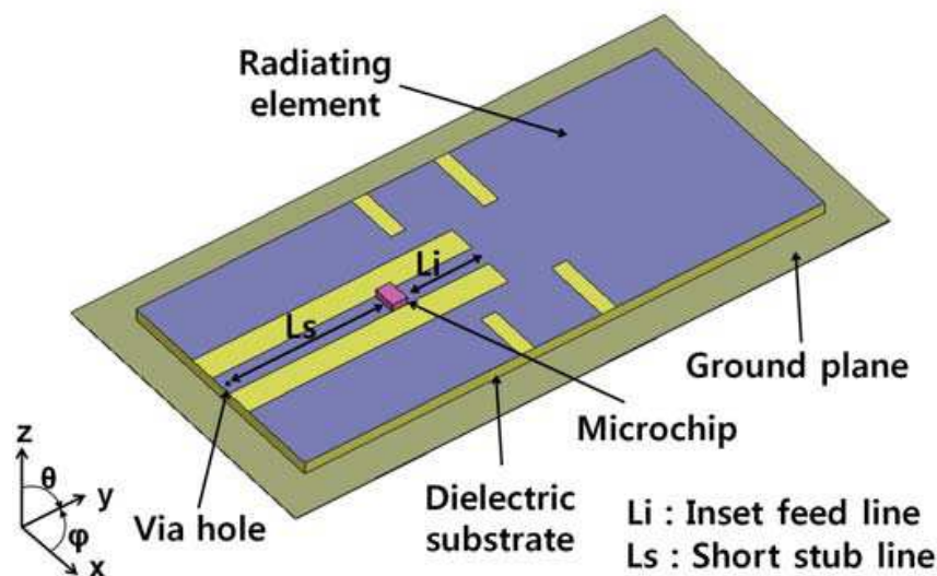
Fig. 4.7 Structure of the compact patch-type tag antenna
