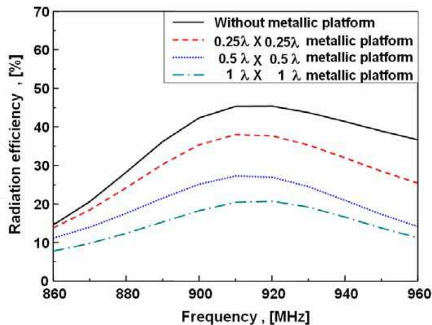
Fig. 4.4 Simulated radiation efficiency for different sizes of metallic platforms
