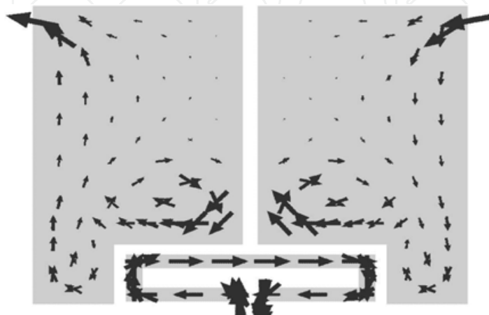
Fig. 4.3 Surface current distribution of balanced-type microstrip patches
