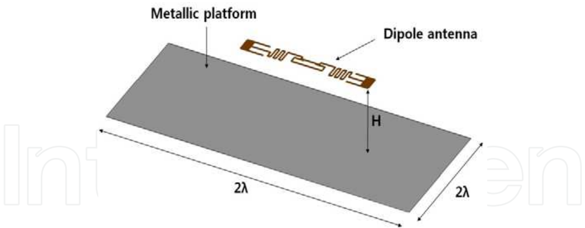
Fig. 3.1 Conventional dipole tag antenna above the metallic platform
