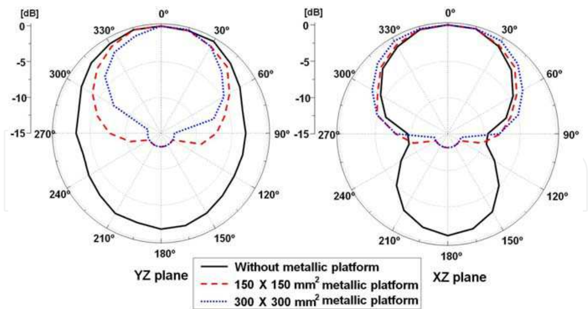
Fig. 4.6 Measured radiation patterns with different sizes of metallic platforms
