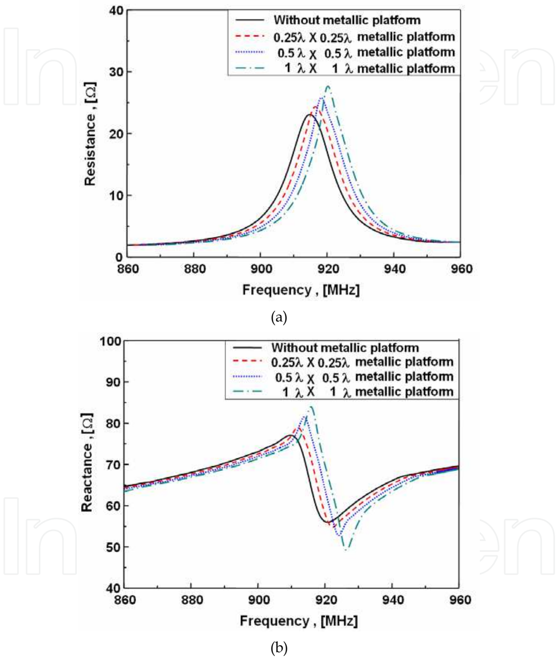
Fig. 4.8 Simulated impedance characteristics for different sizes of metallic platforms Fig. 4.8 shows the simulated impedance characteristics of a compact tag antenna with different sizes of metallic platforms. It is noticed that the impedance variation is small without metallic platform and with various sizes of metallic platforms. Therefore, the impedance has very good tolerance for different sizes of metallic platforms. Fig. 4.9 shows
