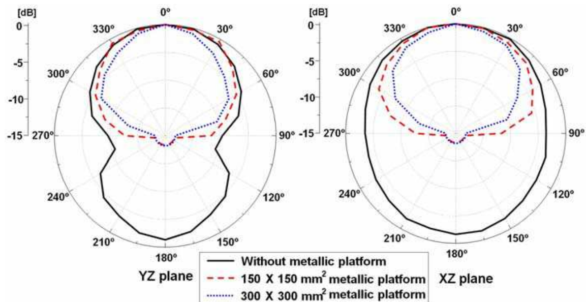
Fig. 4.11 Measured radiation patterns with different sizes of metallic platforms
