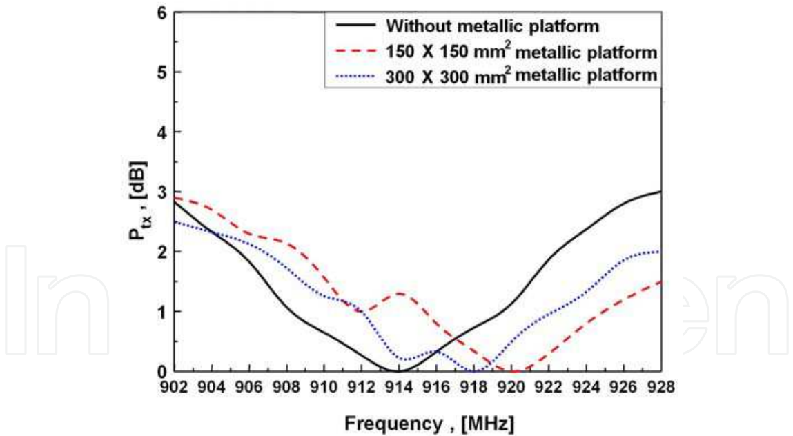
Fig. 4.10 Measured power bandwidth versus the different sizes of the metallic platforms Fig. 4.10 shows the measured power bandwidth versus frequency when the tag is mounted on different sizes of metallic platforms. The bandwidth within 3 dB power variation for the square metallic platform of 150 ~ 300 mm length remains good. So, the bandwidth has a very good tolerance for the large sized metallic platforms. Fig. 4.11 shows the measured radiation patterns. It is shown that the direction of the antenna main beam does not vary
