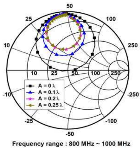
Fig. 3.6 Impedance characteristic with varying the size of the metallic platform
