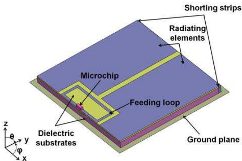
Fig. 4.1 Structure of the balanced-type microstrip patches for tag antennas
