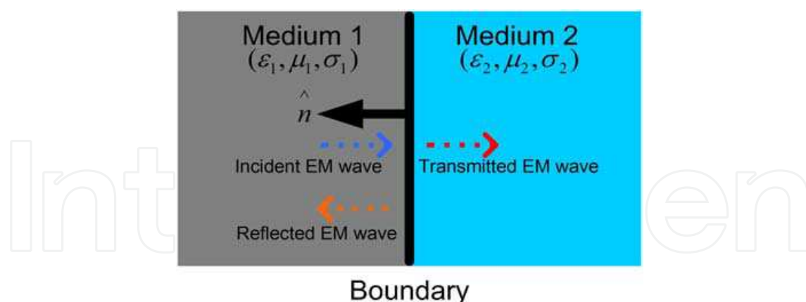
Fig. 2.1 Electromagnetic boundary between two media
