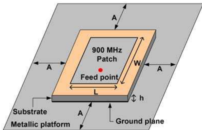
Fig. 3.5 Microstip patch antenna mounted on the metallic platform
