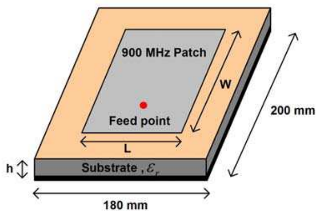
Fig. 3.4 Conventional microstrip patch antenna operating at 900 MHz
