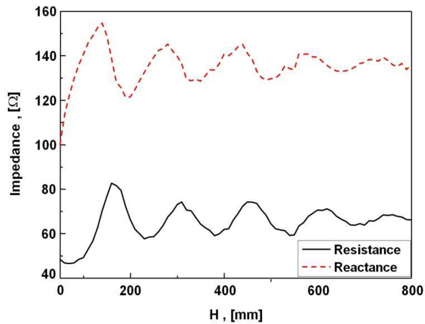
Fig. 3.2 Impedance variation as a function of the distance ( H ) between a dipole antenna and a metallic platform at UHF band
