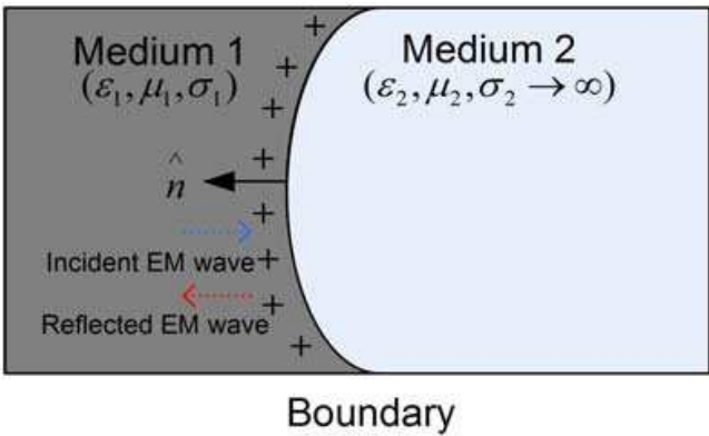
Fig. 2.2 Boundary conditions at the interface of PEC If medium 2 is a PEC with infinite conductivity, all field components must be zero inside of the PEC. Then, we can express the boundary conditions at the interface as follows:
