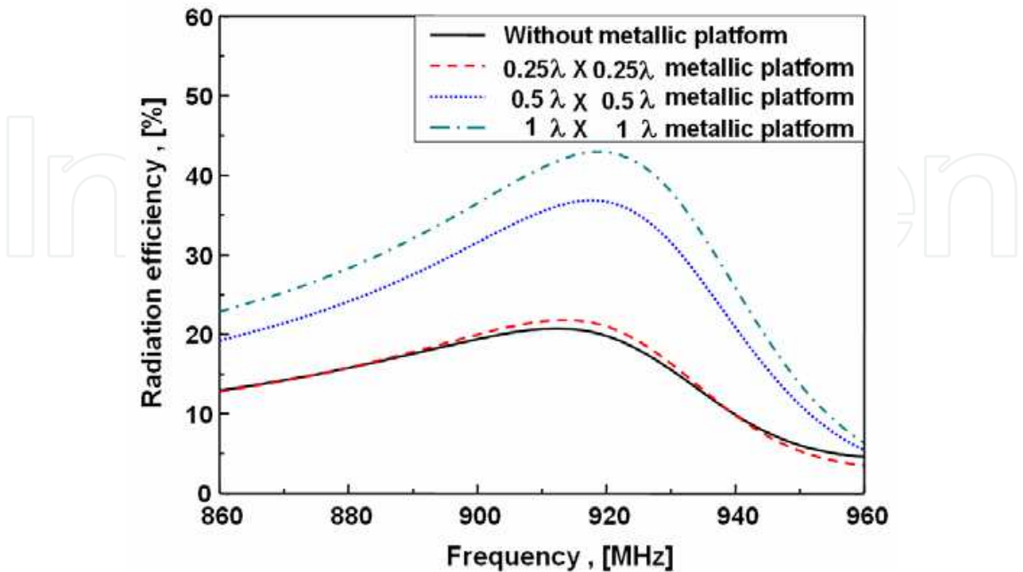
Fig. 4.9 Simulated radiation efficiency for different sizes of metallic platforms
