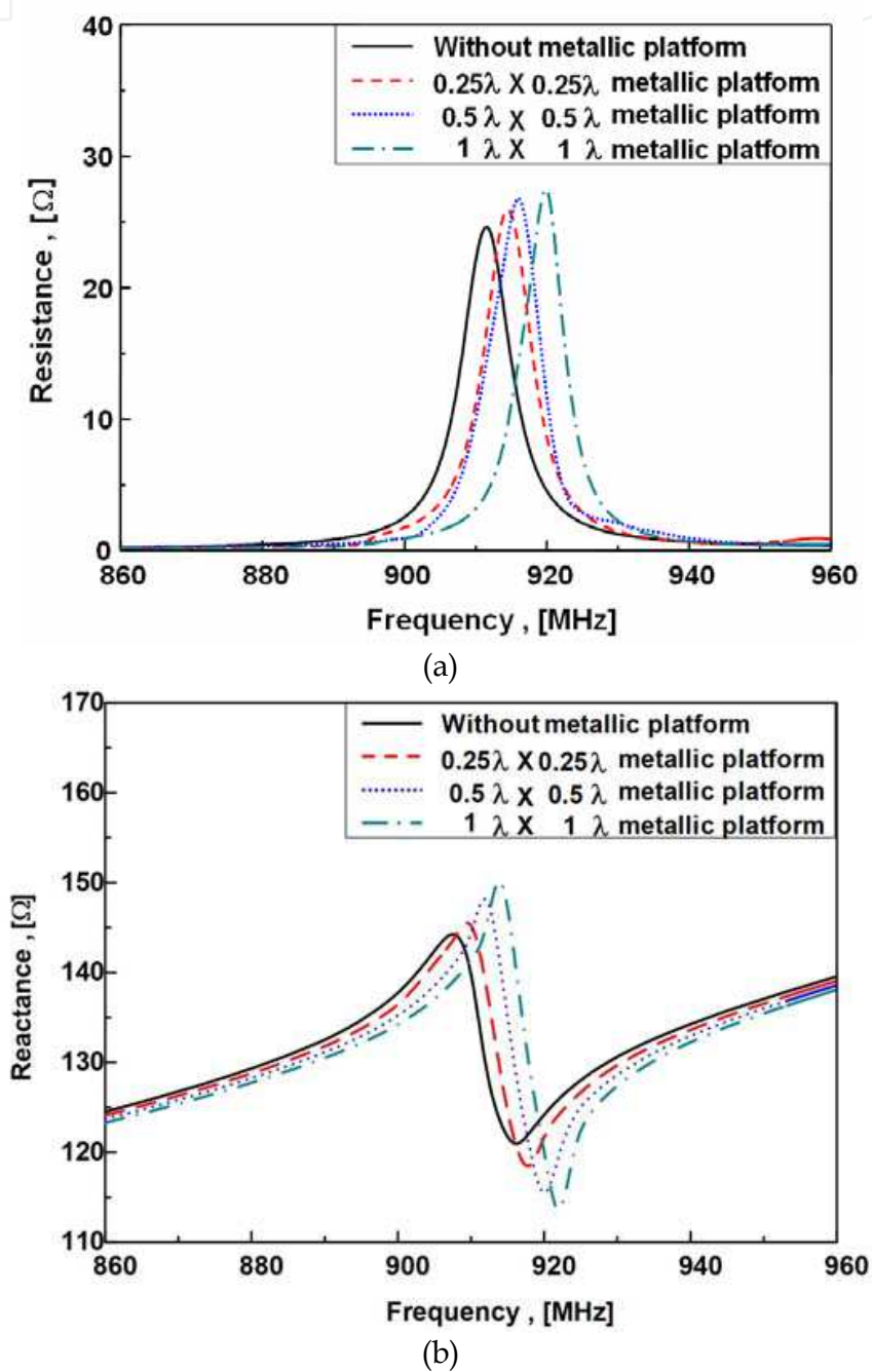
Fig. 4.2 Simulated impedance characteristics with different sizes of metallic platforms
