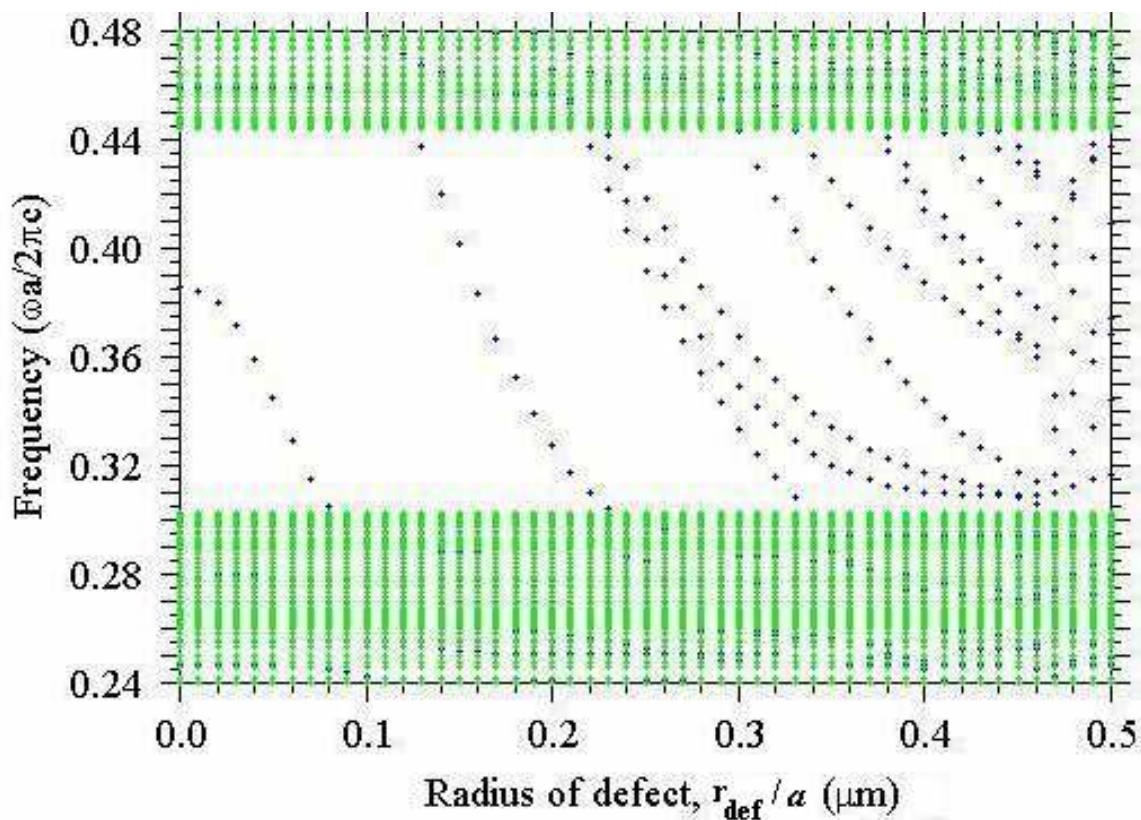
Fig. 6. A plot of the TM modes in rectangular silicon pillars in air with r = 0.18a . The photonic band gap is the white space between green block. The localized modes are shown as blue dotted lines. We create the defect cavity filling in a single silicon pillar.
