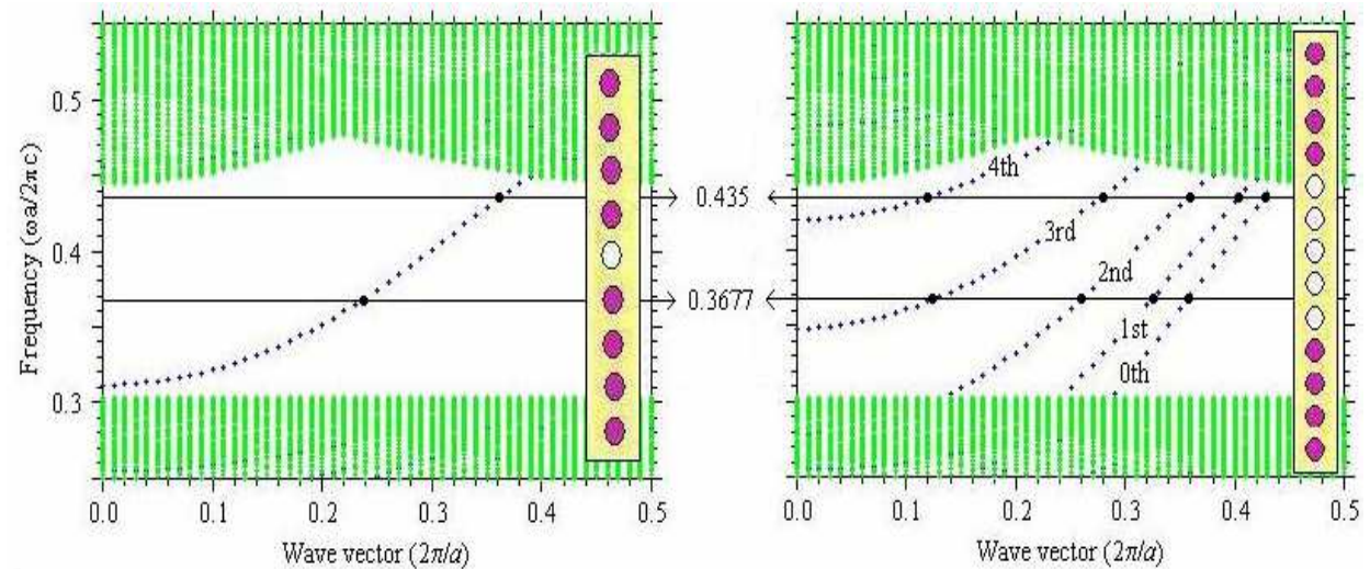
Fig. 20. (a) The dispersion curve for the access PhCW and the computational super-cell (inset). The access PhCW ensures single-mode operation from 0.312(a/\lambda) to the top band gap. (b) The dispersion curve for the multi-mode PhCW and the computational super-cell (inset). The multi-mode PhCW supports 4 guided modes at 0.37(a/\lambda) and 5 guided modes at 0.43(a/\lambda)
