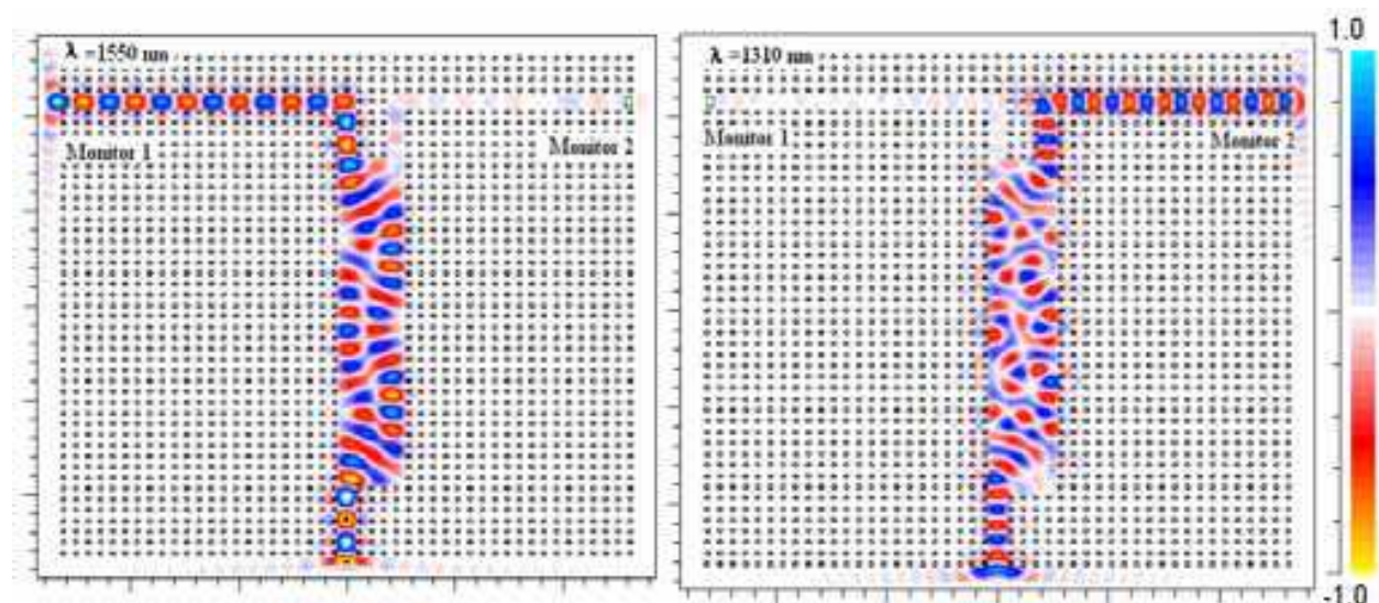
Fig. 25. Steady-state electric field distributions in the designed PhC wavelength DEMUX/MUX MMI based at 1550 nm (left) and at 1310 nm (right).
