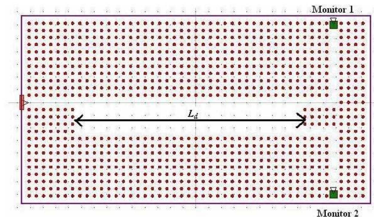
Fig. 24. The designed PhCW DEMUX/MUX MMI based.
