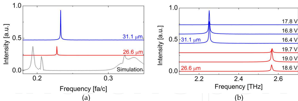
Fig. 7. (a) Simulated and recorded spectra for the active PhC laser Benz, Deutsch, Fasching, Andrews, Unterrainer, Klang, Schrenk & Strasser (2009). The realised devices are both lasing at the K-point, close to the predicted emission frequency. (b) Measured spectra for different periods of the PhC as a function of the applied bias. Both devices show a stable single-mode emission which is independent of the voltage.
