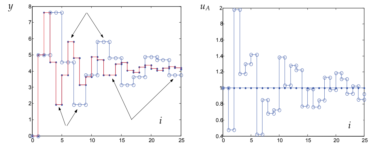
Fig. 3. Left position: the reference response of system (6) to signal u(i)= 1(i) – curve distinguished by “.” - and response of system (6) obtained as output signal of structure in Fig. 2 – curve distinguished by “o”. Note, that consecutive amplitudes of both responses are identical (compare chosen referring amplitudes indicated by arrows). Right position: reference input signal u(i) = 1(i) and input signal u_A(i) of system (6) when included to structure in Fig. 2 as SYSTEM.
