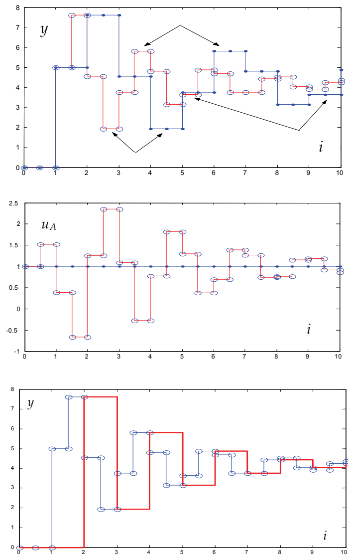
Fig. 5. Upper figure: the reference response of system (6) to signal u(i)=1(i) - curve distinguished by “.” - and the speeded response of system (6) obtained as output signal of structure in Fig. 4 - curve distinguished by “o”. Note, that consecutive amplitudes of both responses are identical (compare chosen referring amplitudes indicated by arrows). Below: reference input u(i)=1(i) and input signal u_A(i) of system (6) when included to structure in Fig. 4 (or in Fig. 2) as SYSTEM. The lowest position: the speeded response of system (6) obtained as output of structure in Fig. 4 - curve distinguished by “o” - and simplified result of scaling with sample time T - heavy line. Note, that every second amplitude of perfectly scaled output y(iT') is equal to respective amplitude of simplified result of scaling for sample time T .
