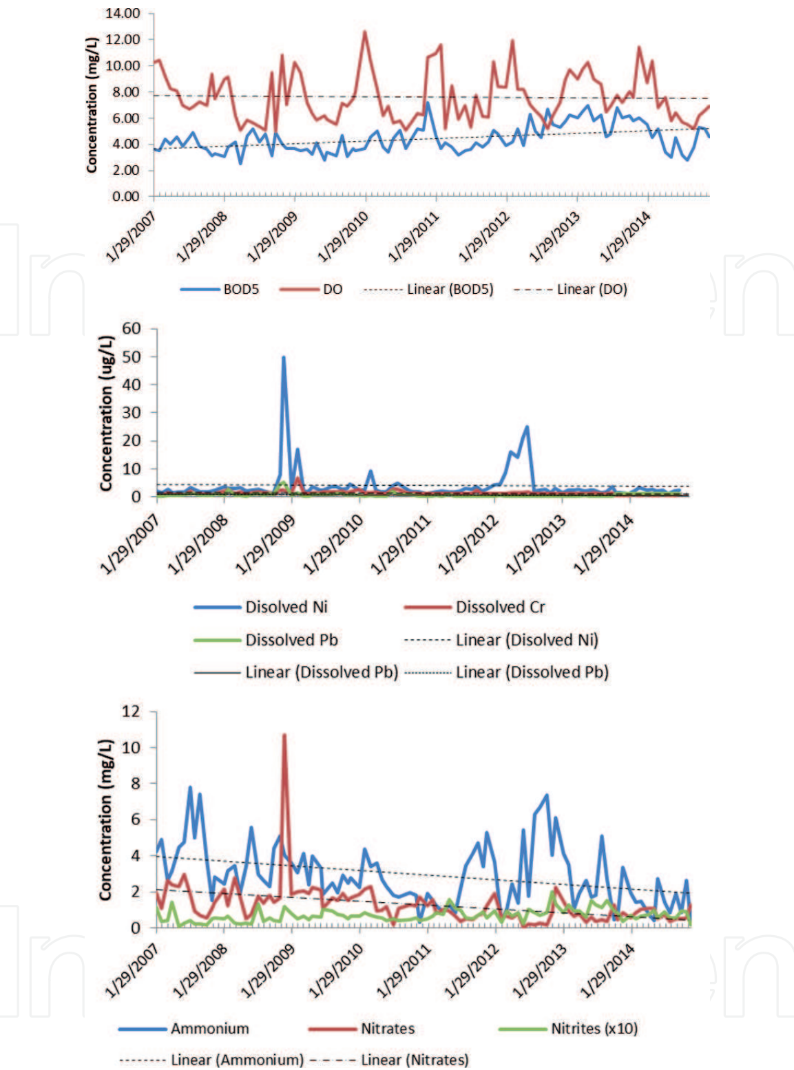
Figure 6. Dynamics of oxygen-related parameters, dissolved heavy metals, and nitrogen nutrients in the monitoring point on Argeş River.
