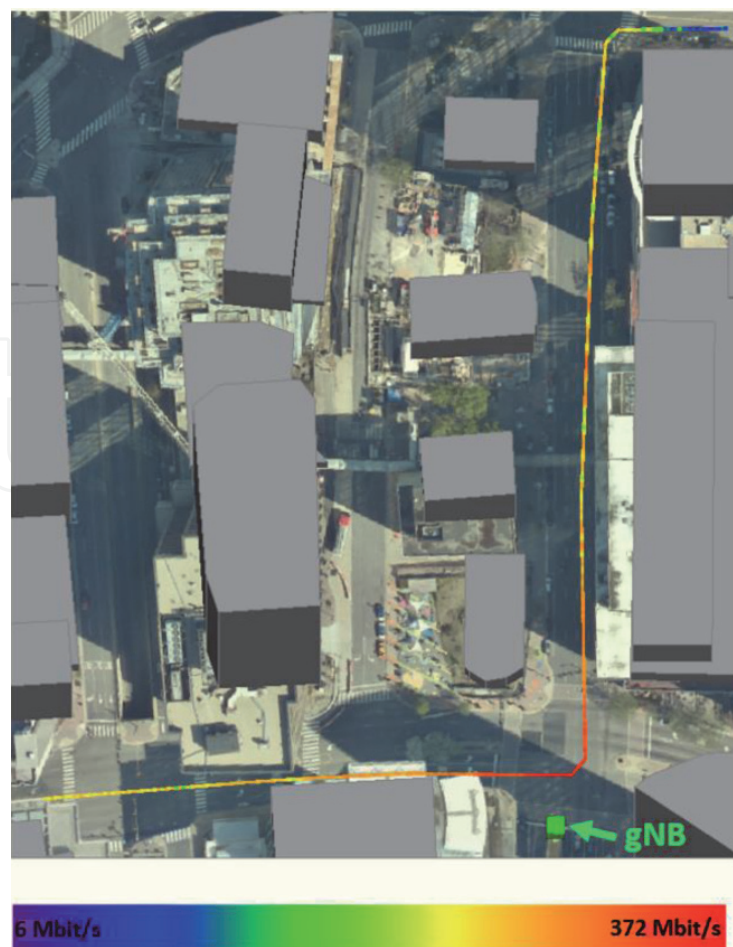
Figure 14. V2X route MIMO channel capacity.
