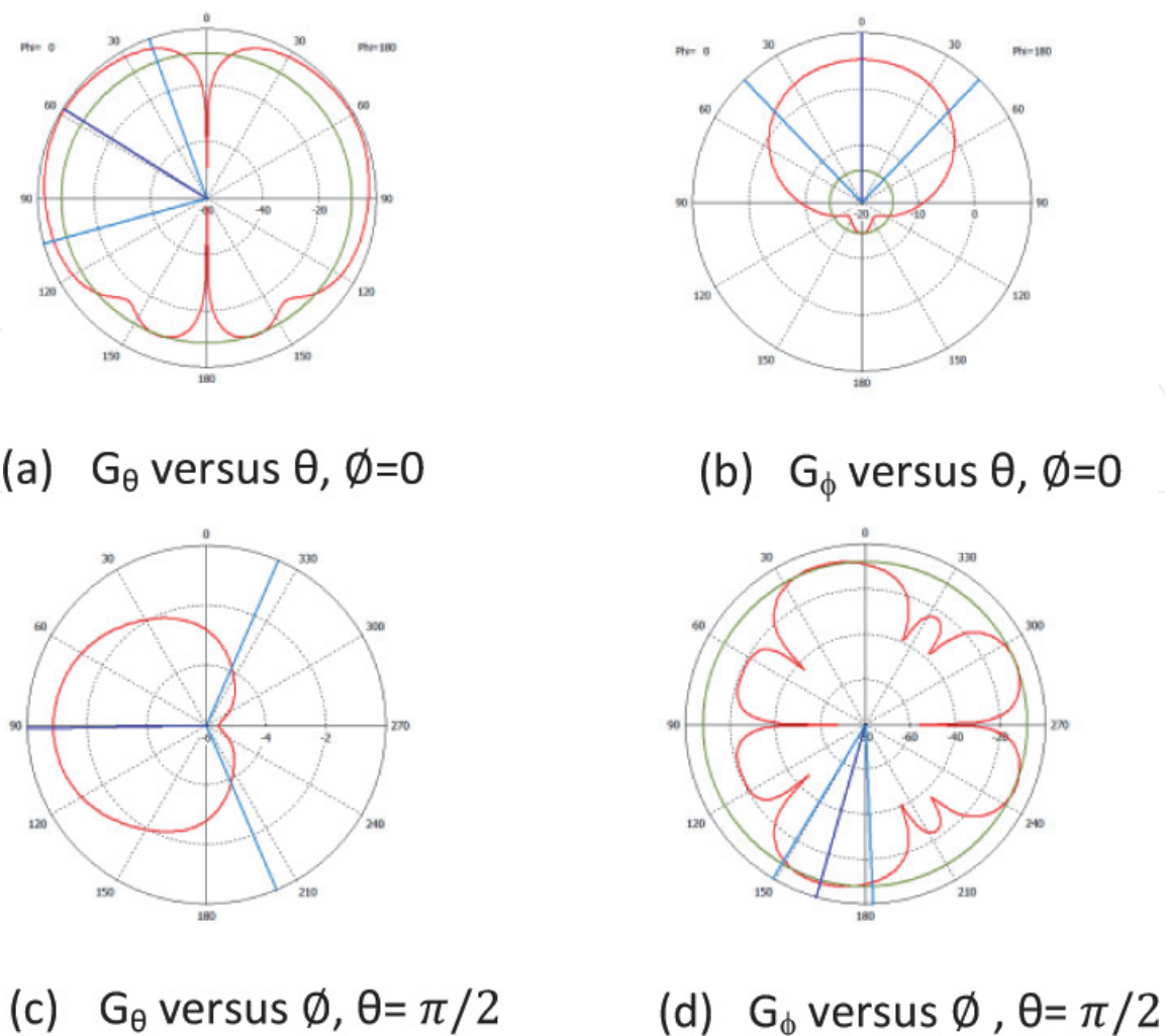
Figure 6. 2D antenna radiation pattern ( \theta is the complement of the elevation angle and \phi is the azimuth angle).
