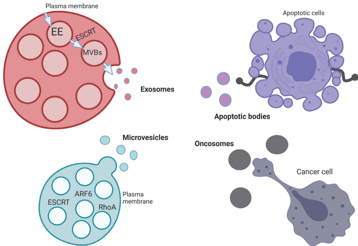
Figure 2. The biogenesis of EVs. (a) Exosomes are produced from early endosomes (EE) and endosomal pathway (ESCRT) and released into extracellular space by fusion of multivesicular bodies (MVBs) with the plasma membrane; (b) microvesicles are produced by direct outward budding of the plasma membrane, with the involvement of cytoskeleton elements (like ARF6 and RhoA) or ESCRT; (c) apoptotic bodies are released into extracellular space by apoptotic cells; (d) oncosomes are secreted by shedding of plasma membrane blebs of cancer cells. Created with BioRender.com (last accessed on September 21, 2021).
