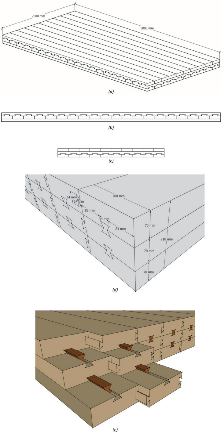
Figure 7. Dovetail wood elements as floor slab alternative-2 (key type): (a) isometric view; (b) front view; (c) side view; (d) with representative dimensions; (e) detail.
