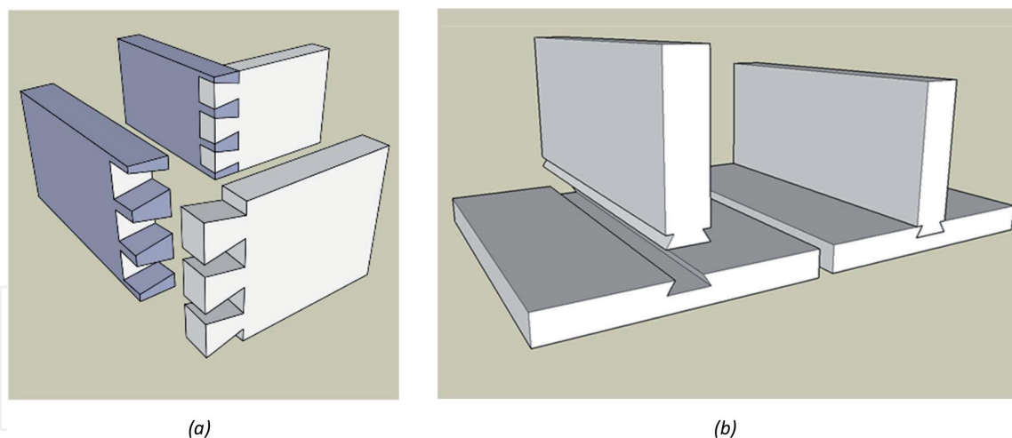
Figure 4. Dovetail joint as one of the oldest joining techniques in furniture design: (a) a through dovetail joint; (b) a sliding dovetail joint (sources: Wikipedia— https://en.wikipedia.org/wiki/Dovetail_joint ).
