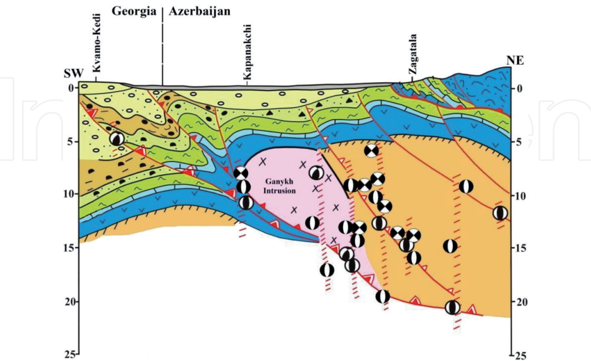
Figure 13. Geological and geophysical section through Zagatala (III-III' in Figure 8, 14), Balakan focal zones of earthquakes—By T.N. Kangarli, F.A. Aliyev, and A.M. Aliyev [23, 28].
