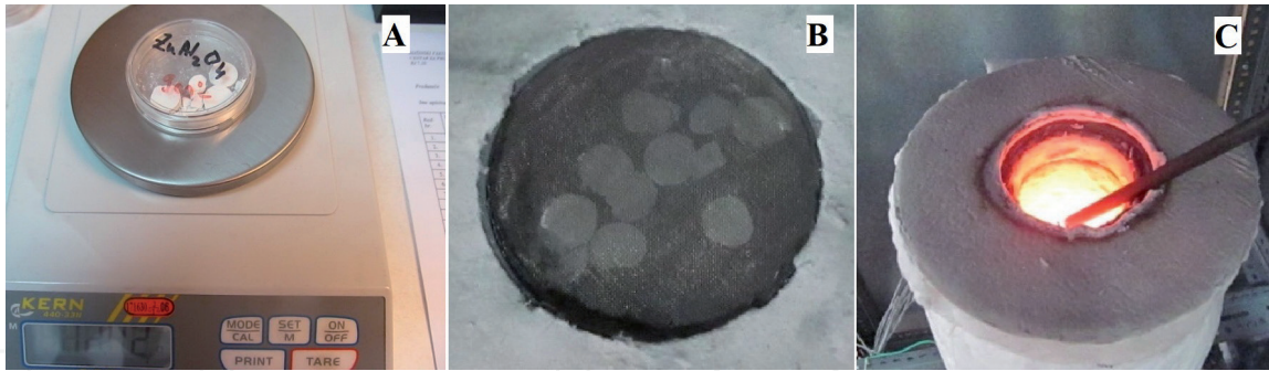
Figure 5. Preparation of \text{ZnAl}_2\text{O}_4 catalysts: A – Weighting; B – Insertion in the metal matrix; C – Initial testing with and without catalysts.
