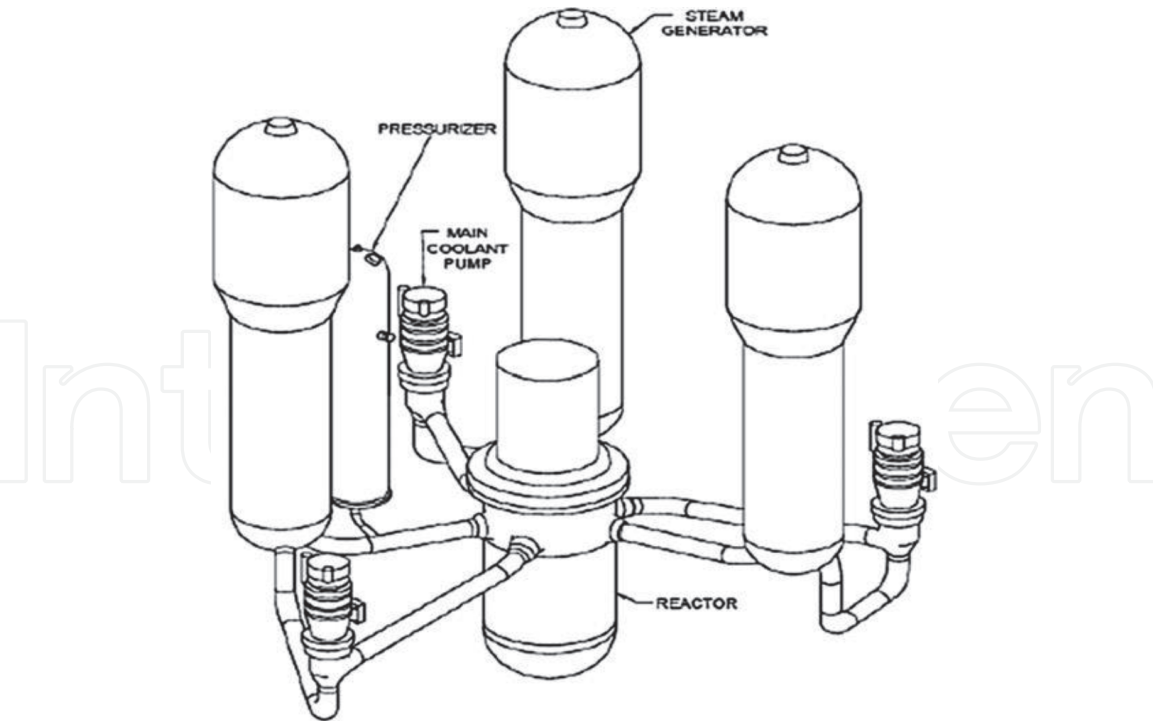
Figure 13. Schematic diagram of three loops PWR reactor coolant system [60].
