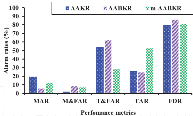
Figure 11. Alarm rates in a steady-state numerical process.
