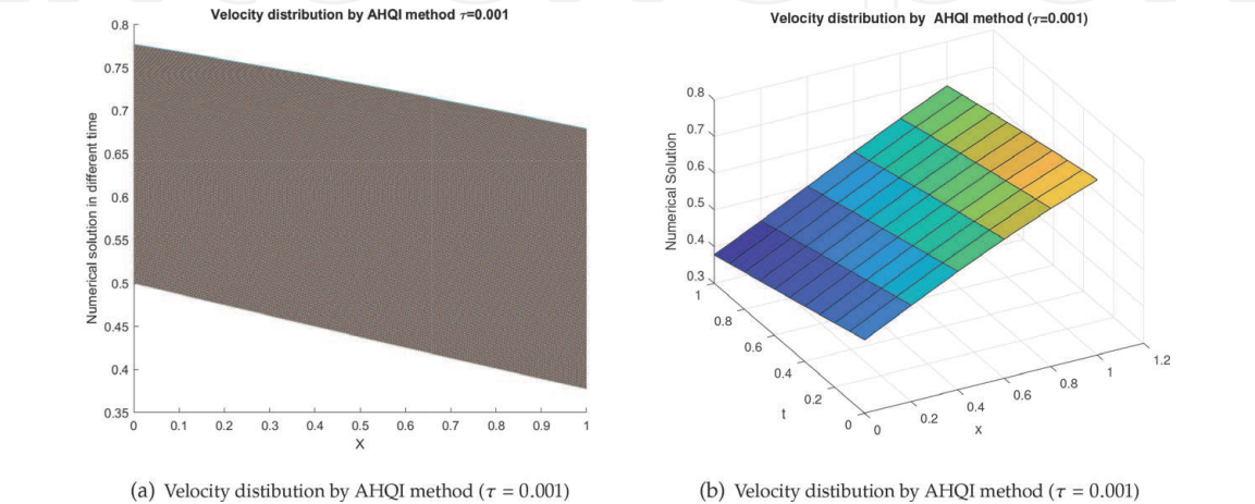
Figure 1. The behavior of numerical results of equation (1) by AHQI for \tau = 0.001 .
