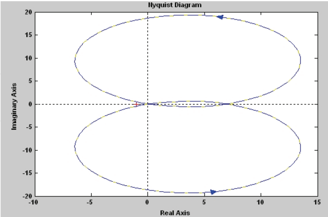
Fig. 14 The Nyquist plot of the simulated system The outputs of the open loop system show the system instability as shown in Fig. 15.
