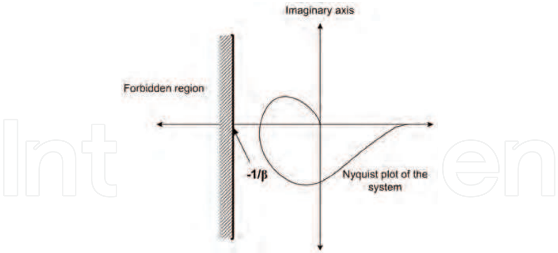
Fig. 6 Nyquist plot with fuzzy feedback system (Ray & Majumderr 1984).
