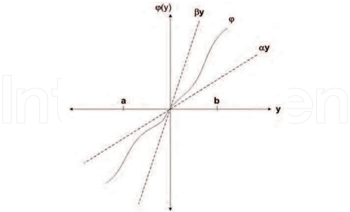
Fig. 5 Sector Bounded Nonlinearity for all t \geq 0 and all y \in [a, b] then: \varphi(y) is a “Sector Nonlinearity”:
