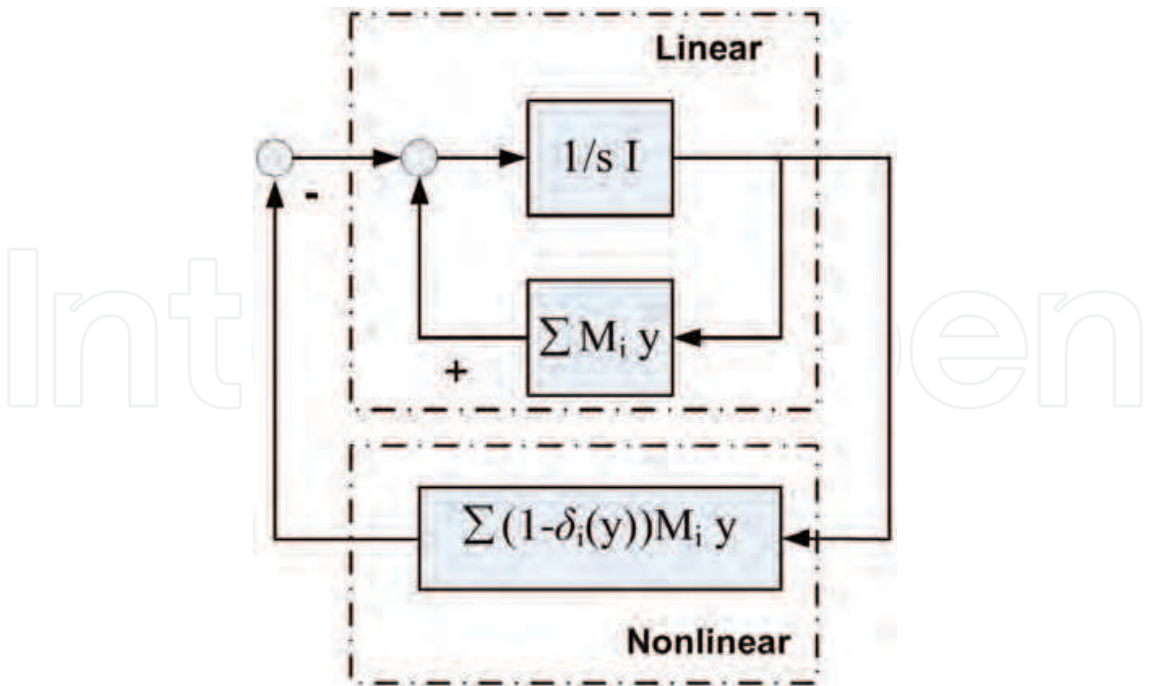
Fig. 4 T-S Fuzzy System according to the structure of the problem of LUR'E If \varphi is bounded within a certain region as shown in Fig. 5 such that there exist:
