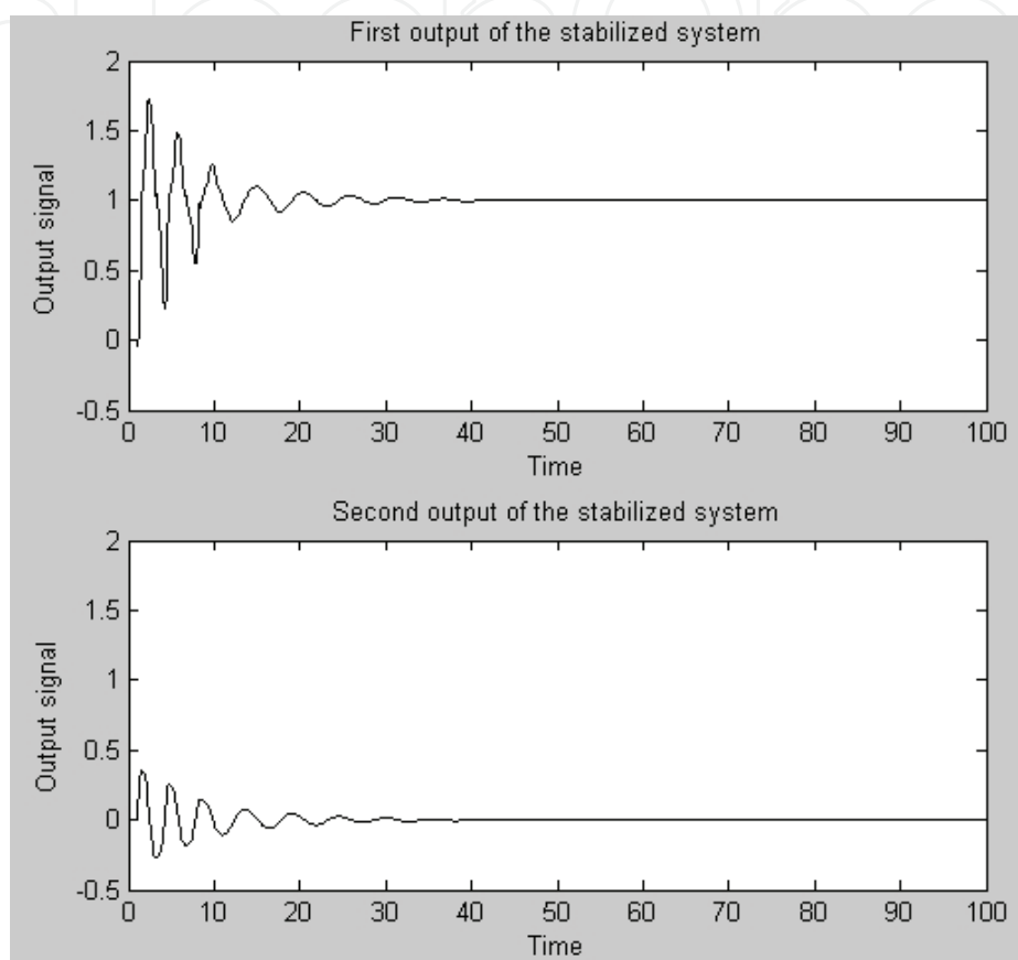
Fig. 16 The outputs of the stabilized simulated system
