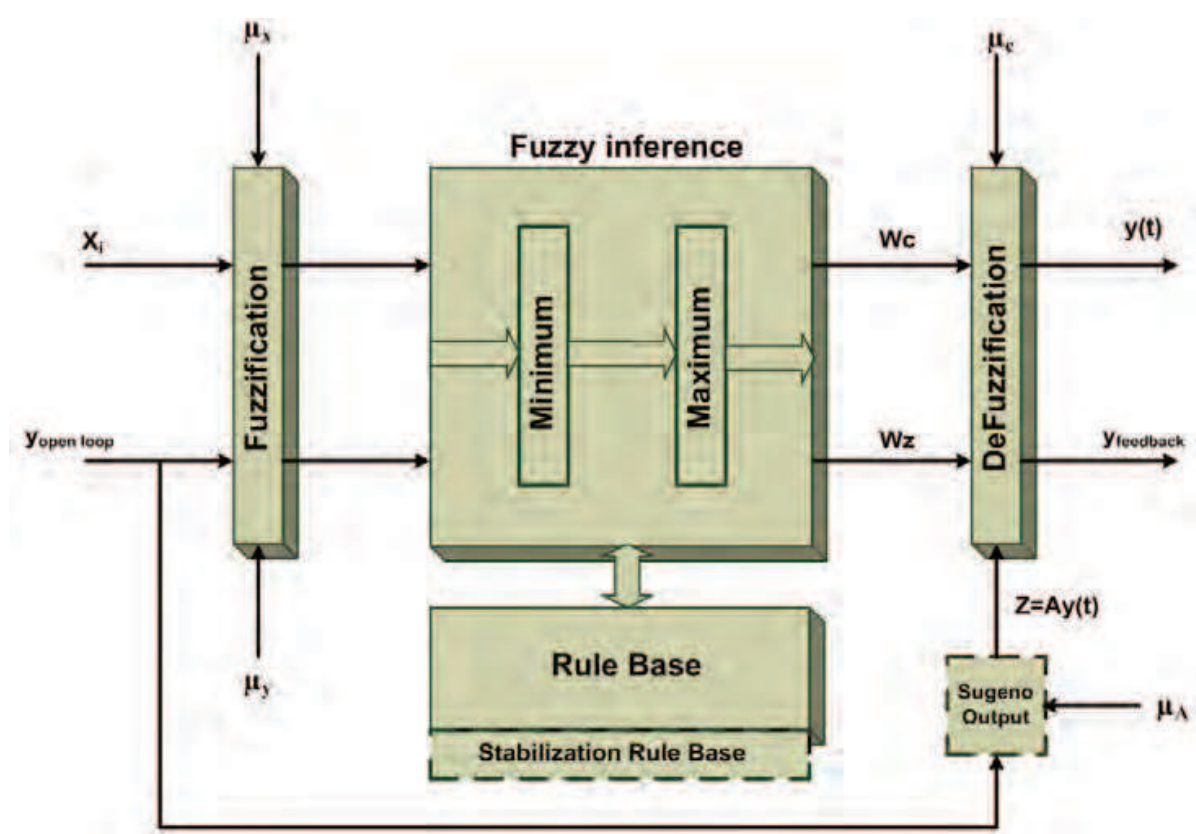
Fig. 8 The modification to the fuzzy system structure
