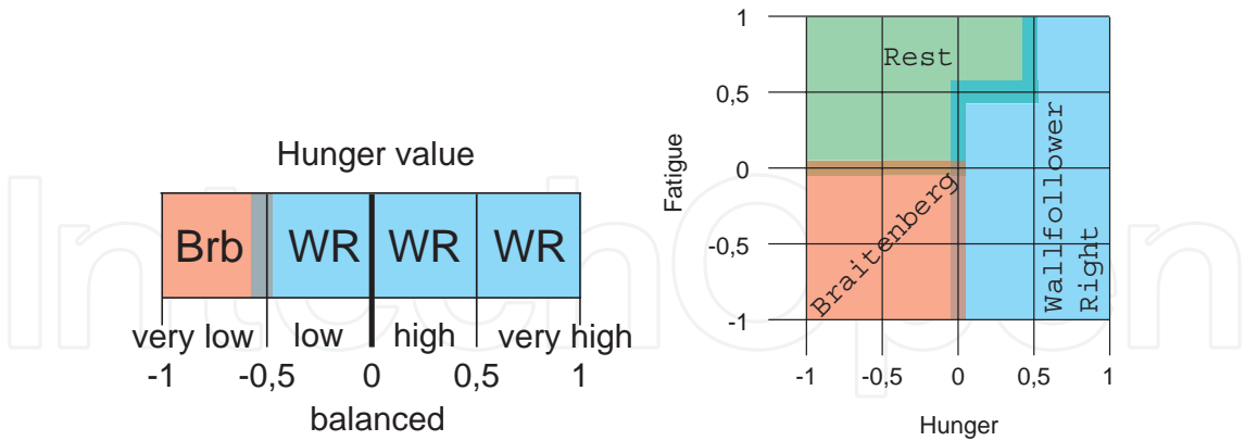
Fig. 3. The quantised internal values (e.g. Hunger and Fatigue) are quantised into four segments; each segment is assigned a behaviour primitive (action selection matrix).
