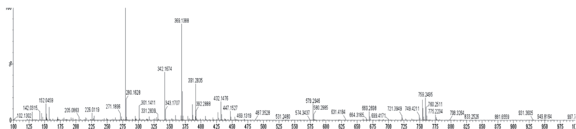
Figure 12. MS spectra.
