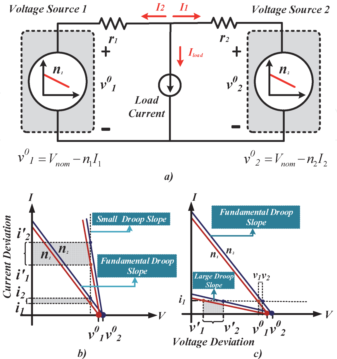
Figure 1. (a) A simple DC MG with two DGs, (b) the effect of small drop causes voltage deviation with current splitting error at full load, and (c) the effect of the large droop gains in voltage deviation with current sharing error under light load conditions, respectively.
