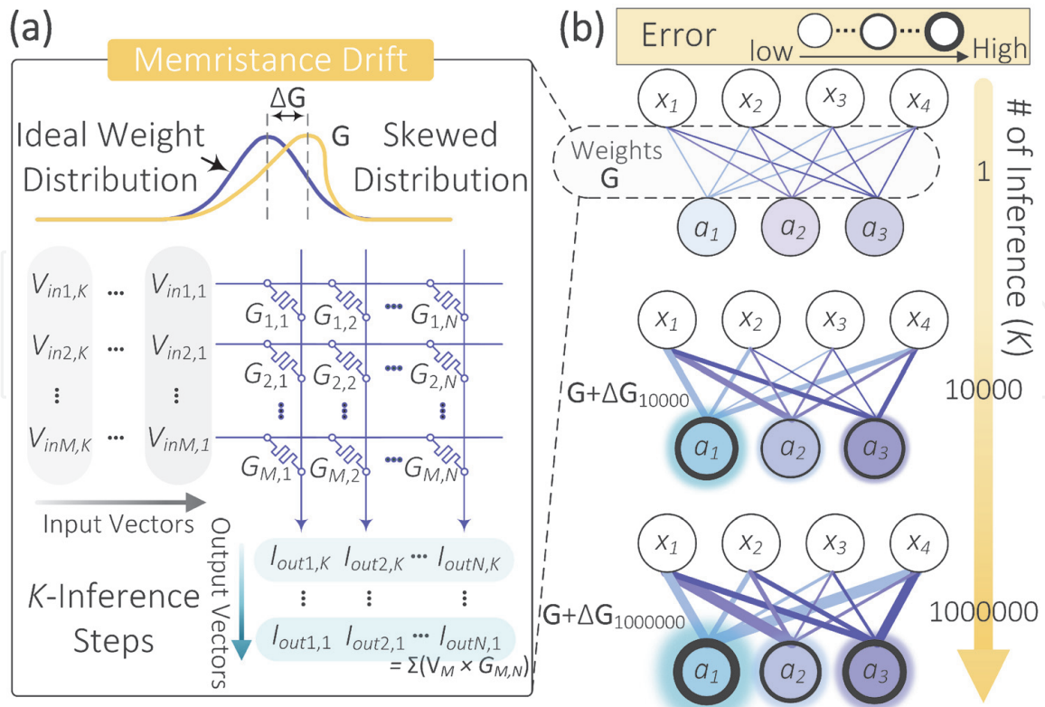
Figure 1. (a) Neural network (NN) weight matrix mapped onto crossbar with conductance matrix G . Each subsequent VMM operation will cause a slight skew in the distribution of the memristors' conductance. (b) Initially, the error due to memristance drift is negligible. Over many inference operations, the skew in the conductance distribution builds up resulting in significant error in the NN output. Figure reprinted by [56].
