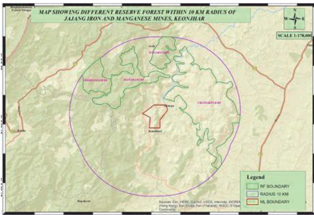
Figure 2. Outline map within 10 km radius of Jajang iron and manganese ore mine at Keonjhar. RF: Reserve Forest, ML: Mining lease.
