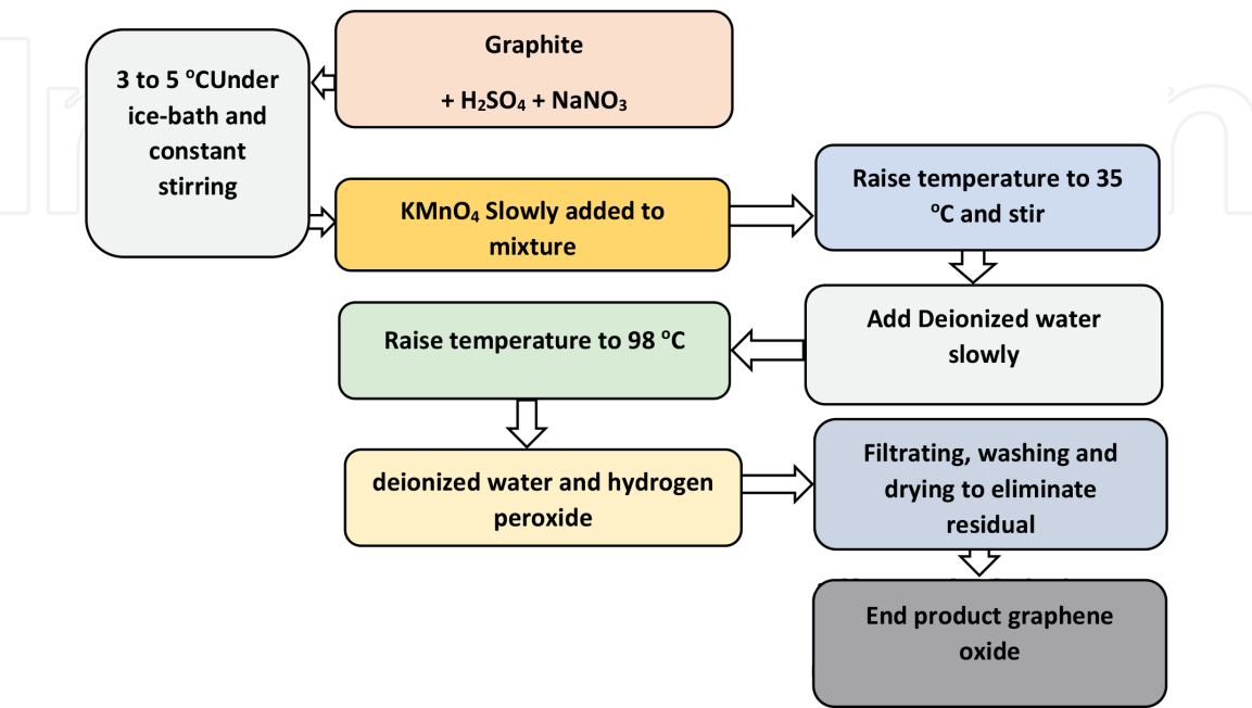
Figure 5. Schematic flow chart of GO synthesis by Hummer's Method.
